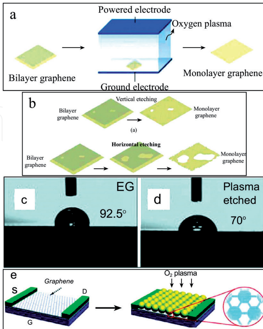
Figure 2. (a) Sequence of graphene etching via O_2 plasma. (b) Schematic of two etching mechanisms of O_2 plasma: vertical etching and horizontal etching. (c, d) The contact angle of graphene/SiC without/with O_2 plasma, respectively. (e) On-chip device assisted by O_2 -etched nanosphere graphene ((a) and (b) are reproduced with permission from [23], Copyright 2014, Springer; (c) and (d) are reproduced with permission from [24], Copyright 2010, American Chemical Society; (e) is reproduced with permission from [25], Copyright 2011, Wiley-VCH Verlag GmbH & Co. KGaA, Weinheim).
