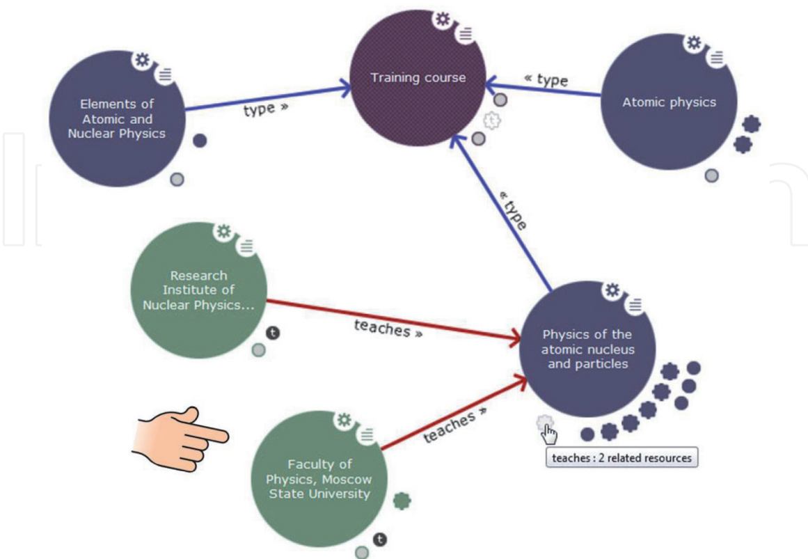
Figure 6. RDF browser: Using the "teaches" property to reduce the number of alternatives under consideration.
