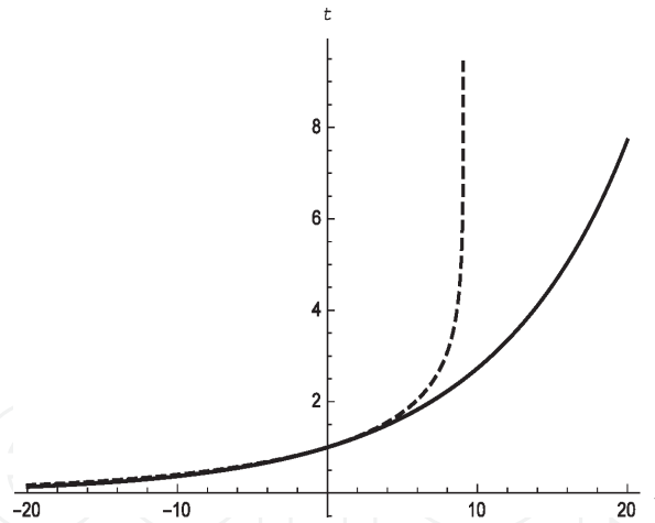
Figure 1. t as a function of s for two values of \tau . \tau = 10 in the solid line and \tau = 1 in the dashed line.
