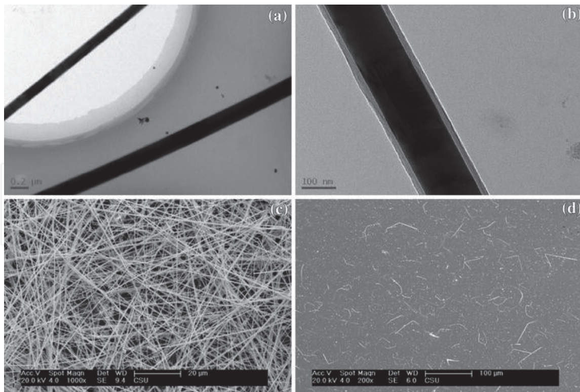
Figure 10. (a) TEM image of core-shell structured AgNW. (b) TEM image of an individual AgNW. (c) SEM image of core-shell structured AgNW. (d) SEM image of AgNW/PI hybrid film [35].
