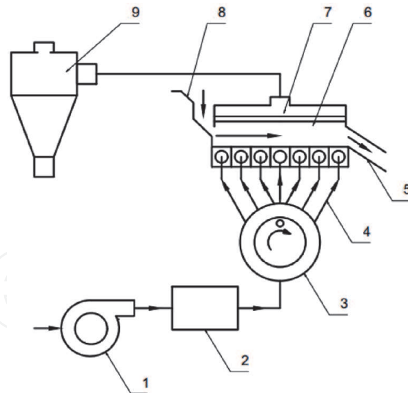
Figure 4. The model of continuous fluidized bed dryer used in experiments. 1. Air fan; 2. heating chamber; 3. air supplier; 4. air duct; 5. product outlet; 6. drying chamber; 7. dust separation chamber; 8. inlet feeder; 9. cyclone dust collector.
