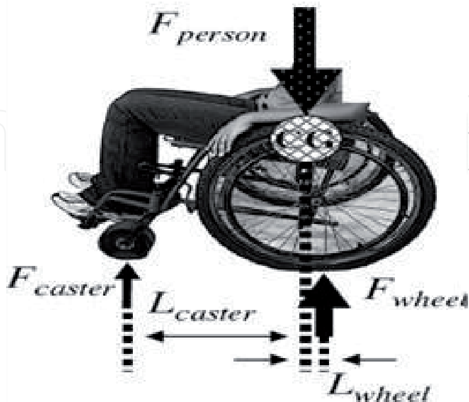
Figure 9. Force analysis [3, 13].
