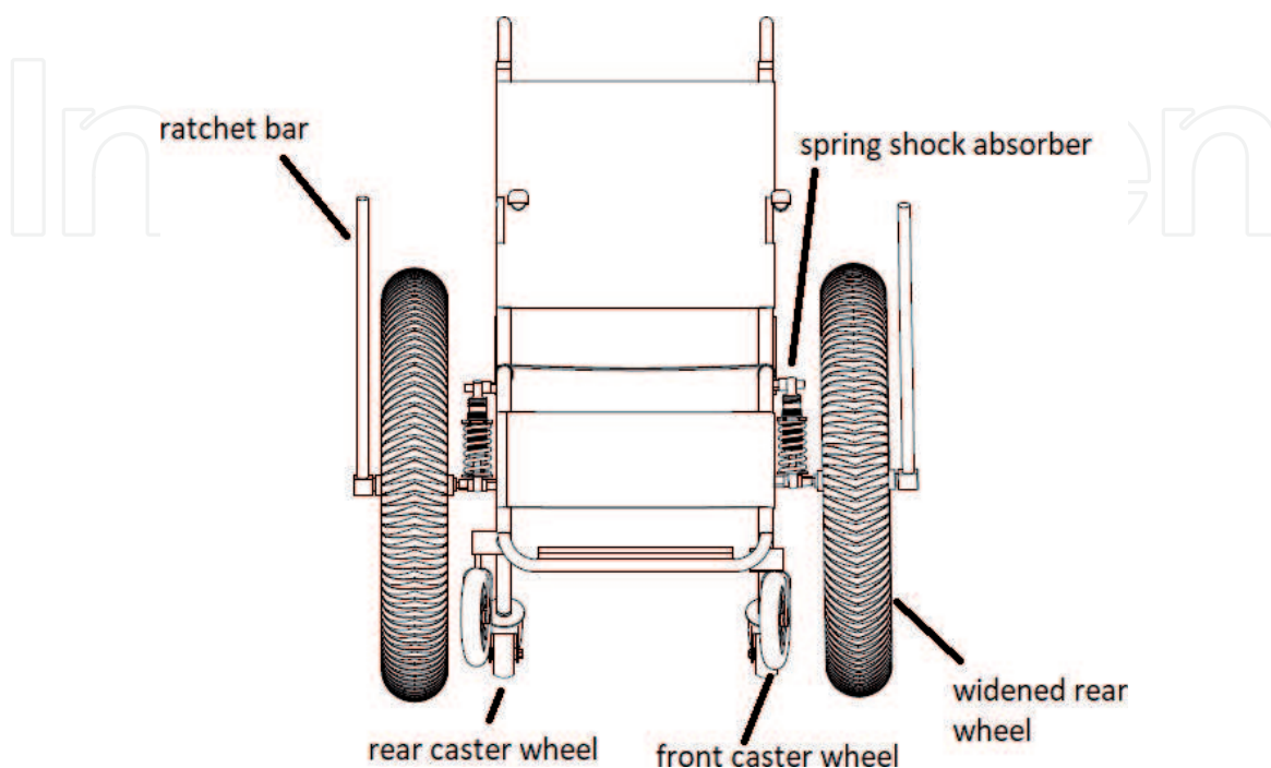
Figure 8. Detailed design assembly.
