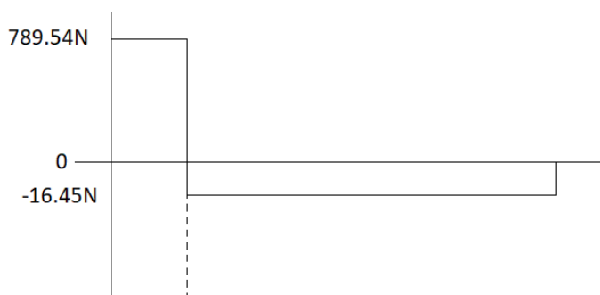
Figure 11. Shear force diagram on the ratchet lever [13].
