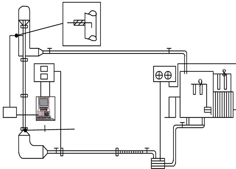
Figure 5. Schematic diagram of two-phase flow experimental facility [18].
