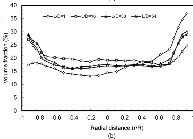
Figure 7. Volume fraction distributions at different (a) L/D for \bar{U}_{ws} = 0.44 m/s and \beta = 9.2\% (solid symbols) and 18.6% (open symbols) [18], (b) L/D for \bar{U}_{ws} = 0.77 m/s and \beta = 18.6\% [18].
