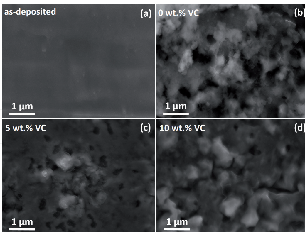
Figure 7. FESEM images of the electrodes surface for (a) as-deposited Ge film, cycled electrodes with (b) 0 wt.%, (c) 5 wt.% and (d) 10 wt.% VC.
