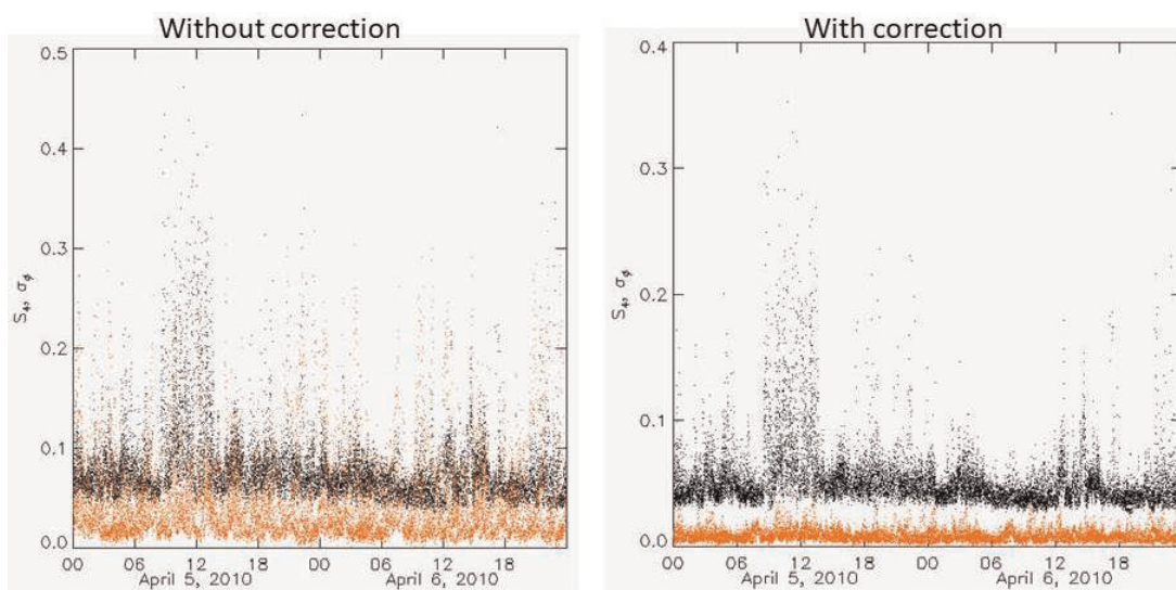
Figure 1. Amplitude (in orange) and phase scintillation (in black) index observations for Hornsund, Svalbard ( 76.9718^\circ N, 15.7844^\circ E), (on left) without geometrical effect correction, (on right) with geometrical effect correction.
