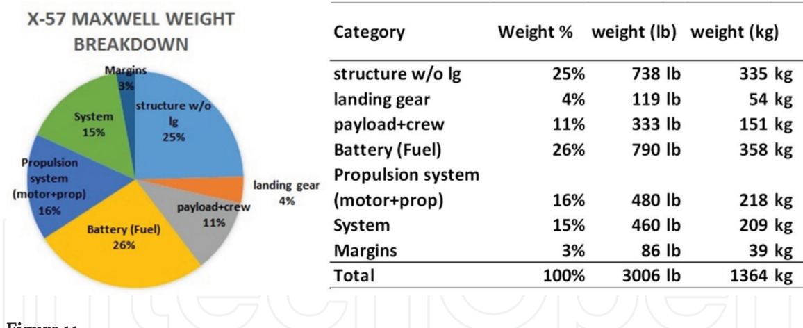
Figure 11. Component weight fractions for the X-57 Maxwell electric distributed propulsion vehicle.
