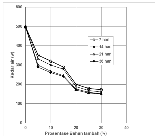
Gambar 2. Hubungan kadar air-prosen bhn tambah – masa peram ( w = 498\% )
