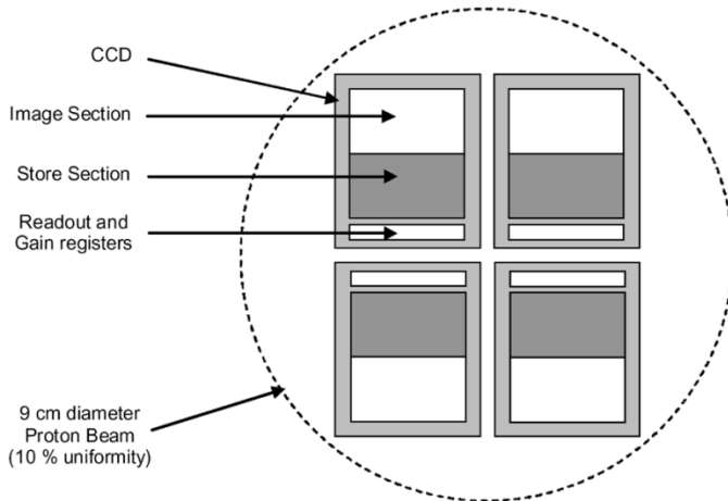
Fig. 7. Irradiation geometry of a single batch of four EMCCDs.
