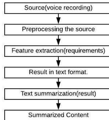
Figure 1. Speech recognition and text summarisation process flow
