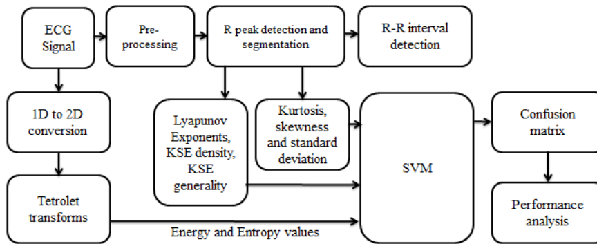
Figure 2. Block diagram of the proposed arrhythmia classification system
