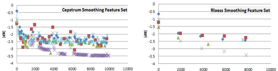
Figure 8. Peak amplitude feature set of cepstrum and roes smoothing
