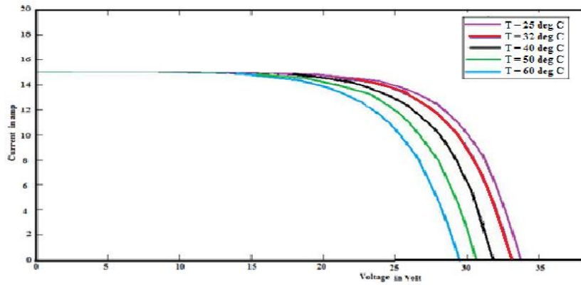
Figure 8. I-V curves for different temperatures at an irradiance of 1000 W/m 2 .
