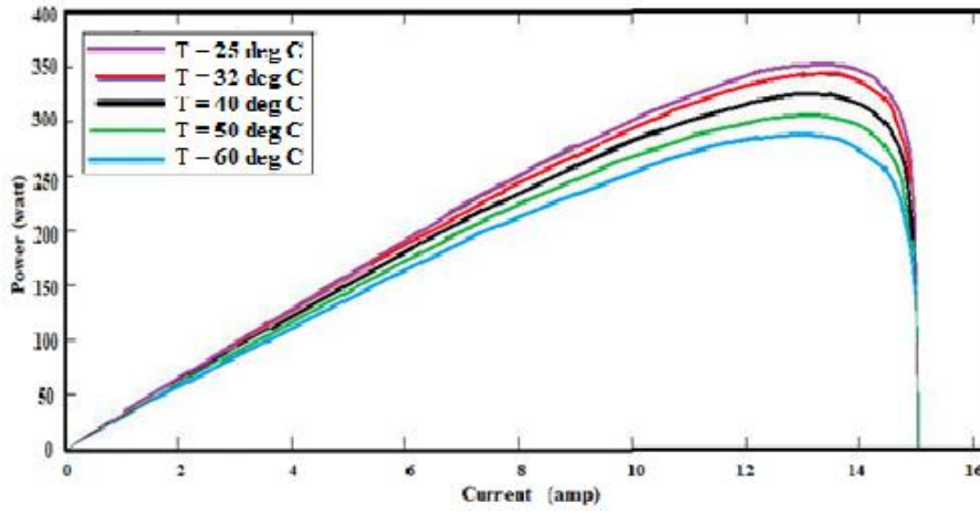
Figure 9. P-I curves (current) for various temperatures at an irradiance of 1000 W/m 2
