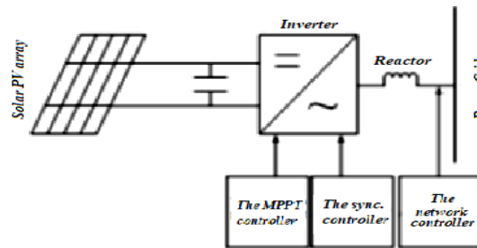
Figure 1. The PV structure system
