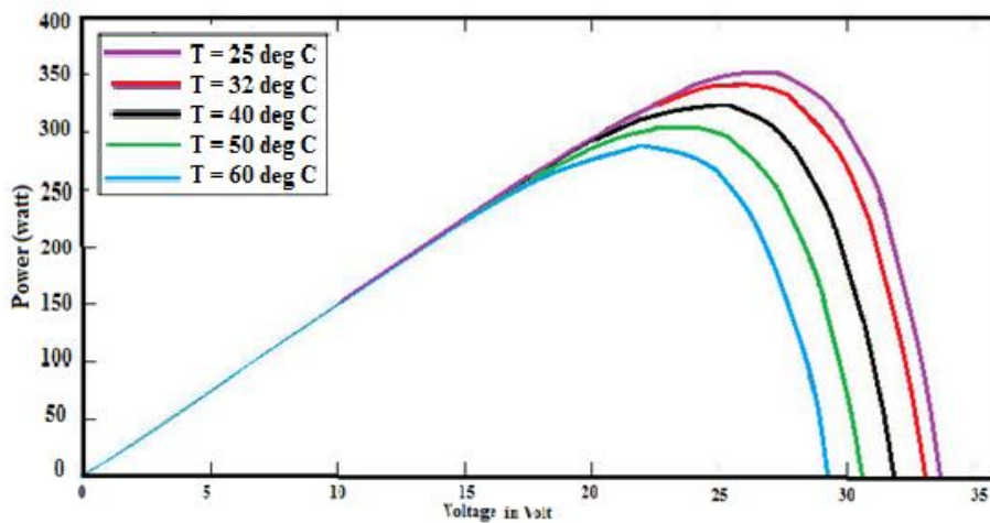
Figure 10. P-V curves (voltage) for various temperatures at irradiance of 1000 W/m 2
