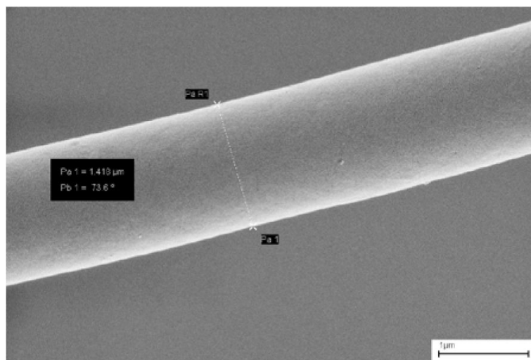
Figure 2. PMMA microfiber presenting a 1.4 μm diameter. Scale bar 1 μm; magnification 19K X
