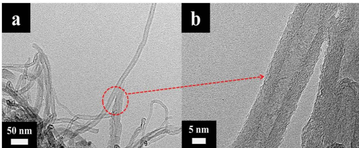
Figure 3. TEM images for pristine MWCNTs (a) agglomerated in bundles, and (b) magnification of the indicated area.
