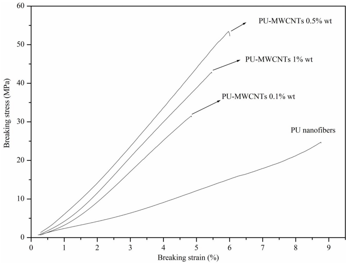
Figure 7. Breaking stress vs. breaking strain curves for PU and PU-MWCNTs nanofibers.
