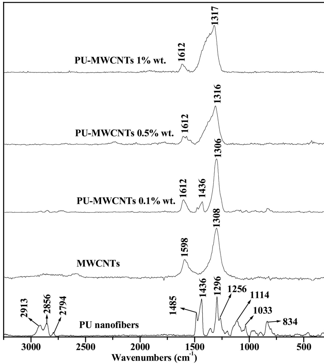
Figure 6. Raman spectra of the polymer nanofiber, MWCNTs, and corresponding nanofibers containing MWCNTs.
