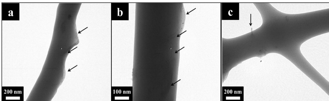
Figure 4. TEM micrographs of (a) and (b) MWCNTs oriented along the PU nanofiber; (c) MWCNT protruding from the PU nanofiber.
