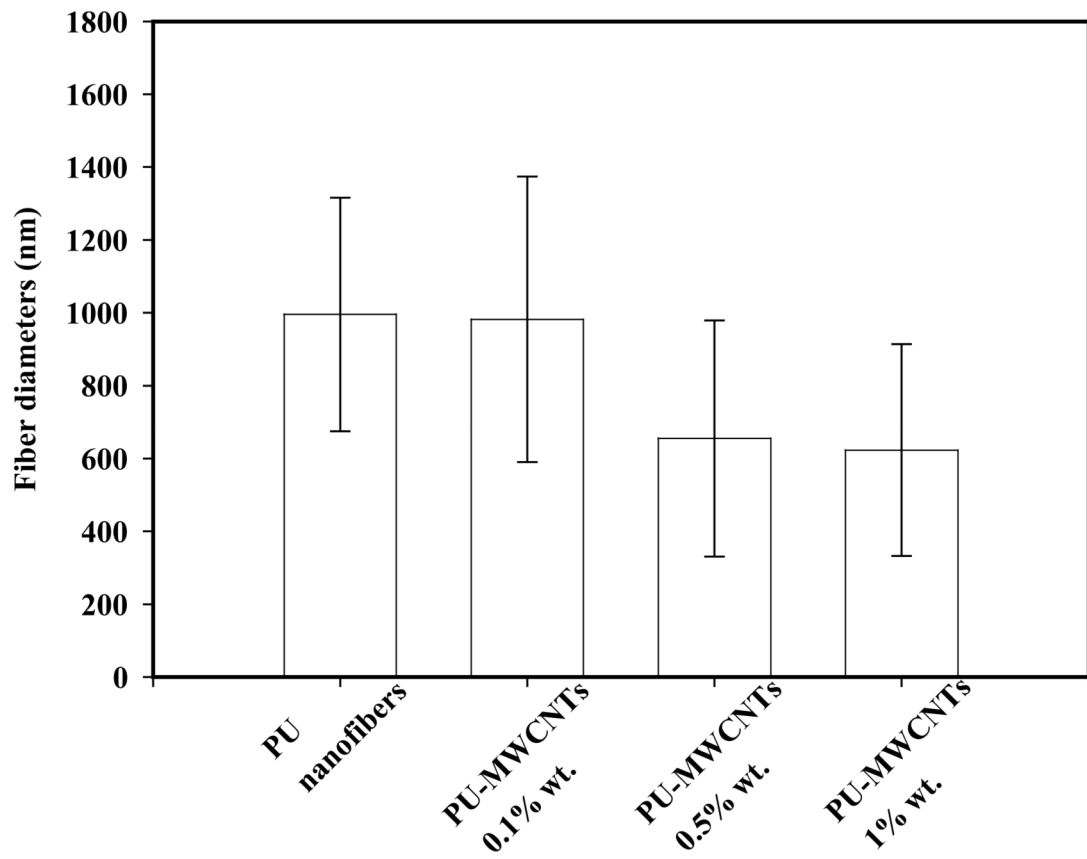
Figure 2. Fiber diameter for PU nanofibers and PU-MWCNTs.
