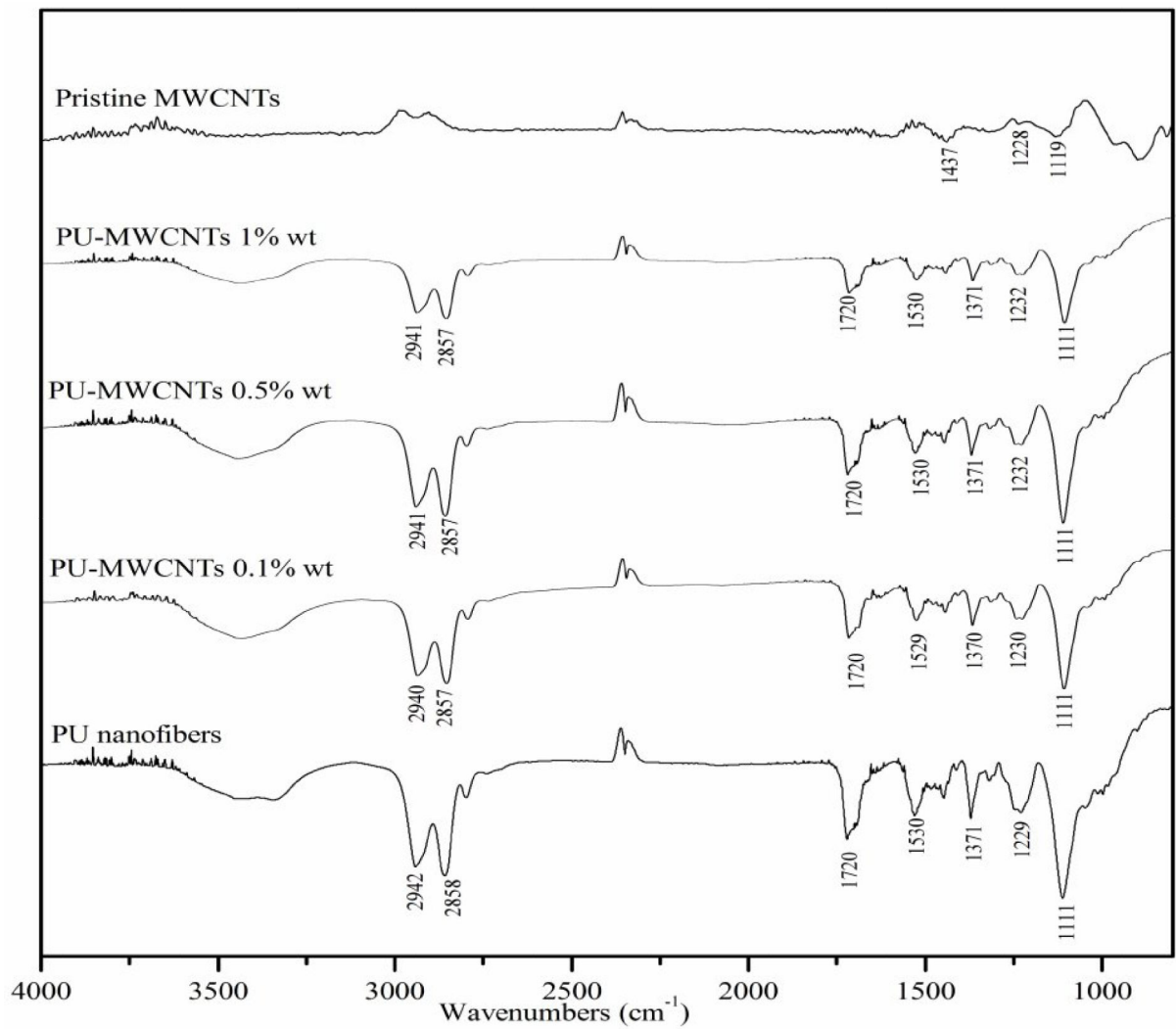
Figure 5. FTIR spectra of MWCNTs, polymer nanofiber and corresponding nanofibers containing MWCNTs.
