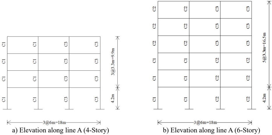
Fig. 2. Configuration of two frames
