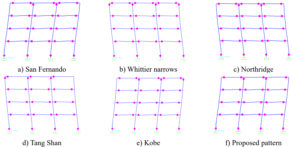
Fig. 13. Distribution of plastic hinge rotations obtained from the SPA procedure and NTHAs in the fringe frame for 4-Story model ( \Delta_{demand} = 66 mm)
