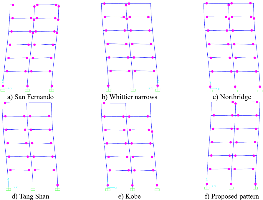
Fig. 14. Distribution of plastic hinge rotations obtained from the SPA procedure and NTHAs in the fringe frame for 6-Story model ( \Delta_{demand} = 82 mm)
