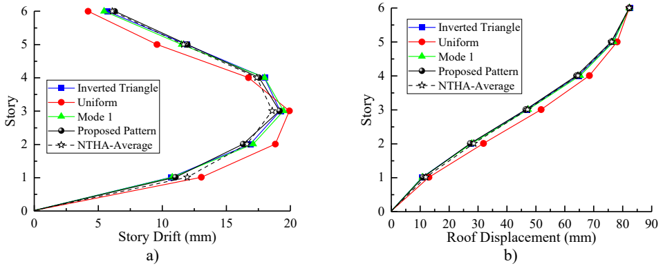
Fig. 7. Comparison of a) peak interstory drifts and b) roof displacements between NSPs and NTHA for 6-Story model
