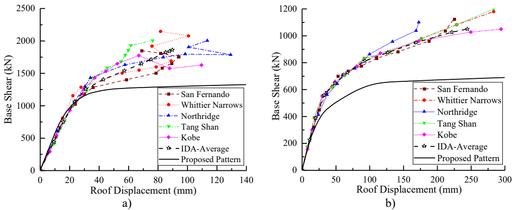
Fig. 8. The capacity curves of a) 4-Story and b) 6-Story models for the proposed load pattern and IDAs
