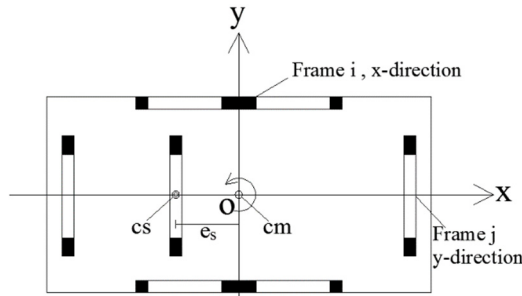
Fig. 1. Typical plan of asymmetric multistory building
