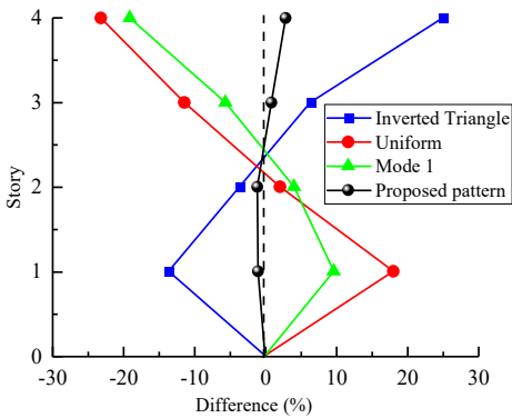
Fig. 11. Differences between different procedures compared with NTHA for 4-Story model
