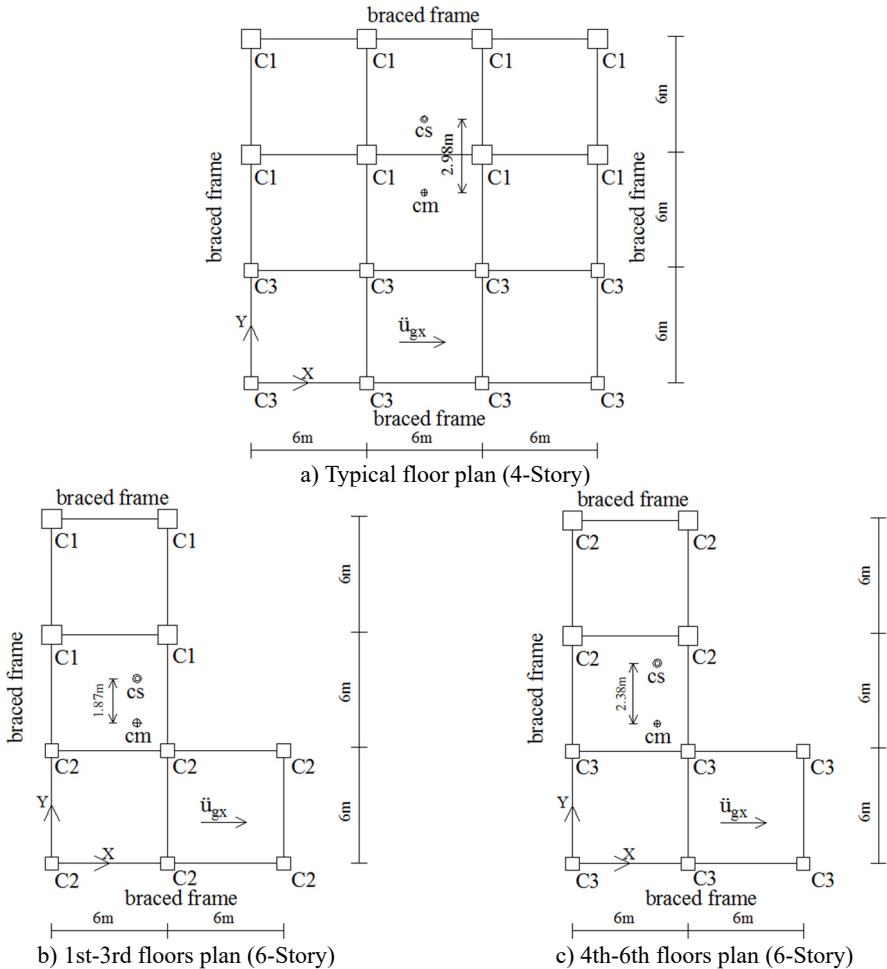
Fig. 3. Typical plan view of two asymmetric buildings
