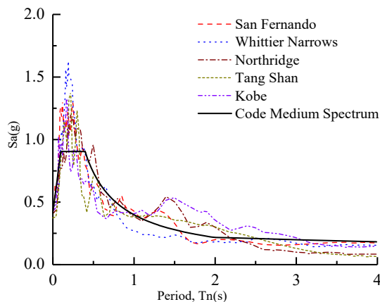
Fig. 4. Scaled pseudo-acceleration response spectra for 5 % damping
