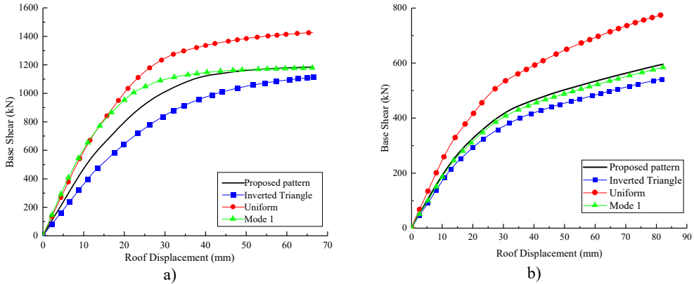
Fig. 5. The pushover curves of a) 4-Story and 6-Story obtained from four different lateral load patterns
