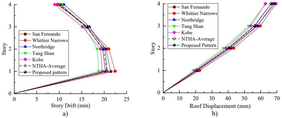
Fig. 9. Nonlinear time history analysis results for 4-story model: a) story drifts, b) roof displacements
