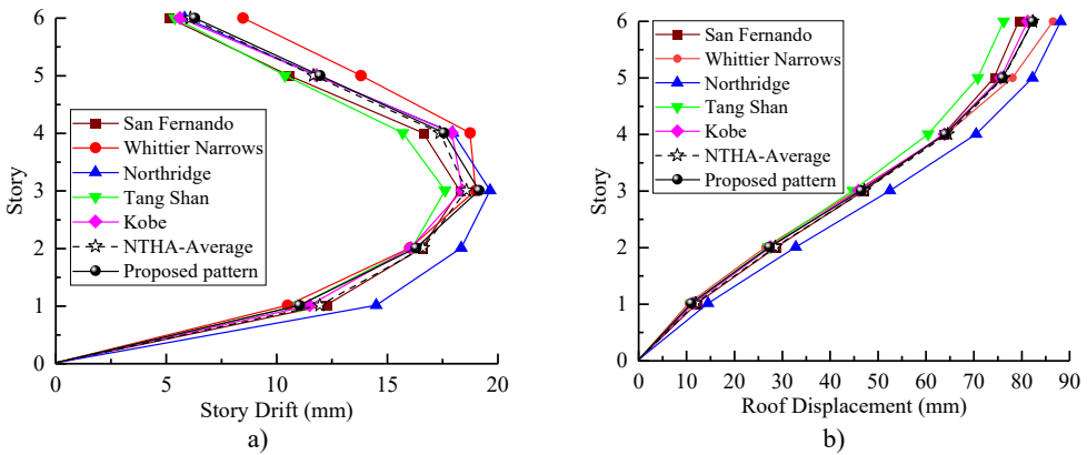
Fig. 10. Nonlinear time history analysis results for 6-story model: a) story drifts, b) roof displacements
