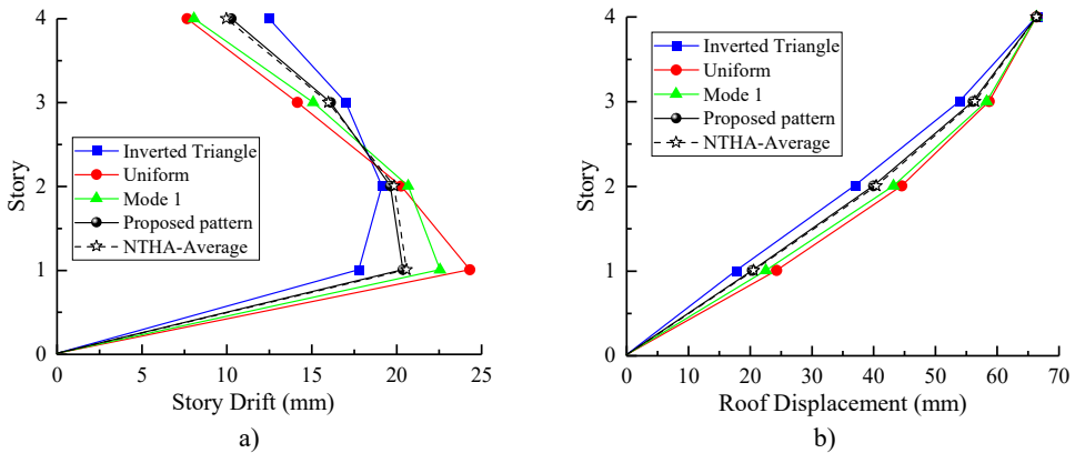
Fig. 6. Comparison of a) peak interstory drifts and b) roof displacements between NSPs and NTHA for 4-Story model
