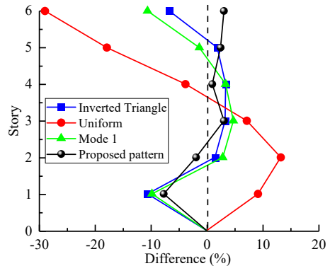
Fig. 12. Differences between different procedures compared with NTHA for 6-Story model
