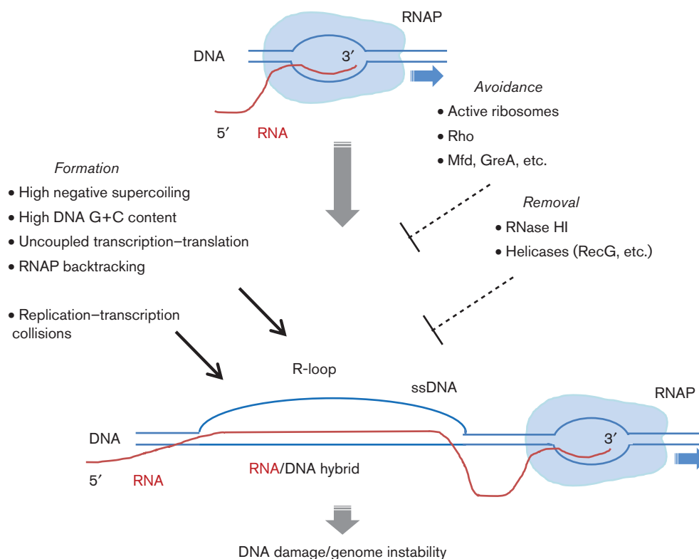
Fig. 2. Schematic representation of R-loop formation. Factors that favour R-loop formation (DNA high negative supercoiling, high DNA G + C content, uncoupled transcription-translation, RNAP backtracking and transcription-replication conflicts) are listed on the left. Anti-backtracking factors preventing R-loop formation (translating ribosomes, Rho, Mfd, GreA) and factors negatively affecting R-loops (RNase HI, helicase RecG active on DNA/DNA and RNA/DNA hybrids) are listed on the right.
