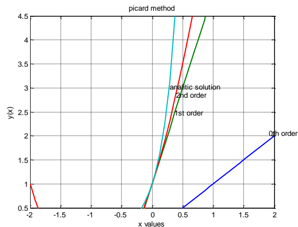
Figure 3.1. Linier IVP Solution Using Picard Method
