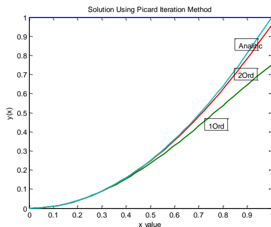
Figure 3.2. Non Linier IVP Solution Using Picard Method
