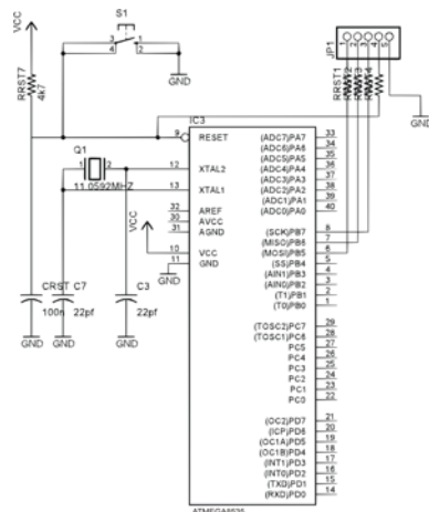
Gambar 2 Minimum sistem ATmega8535
