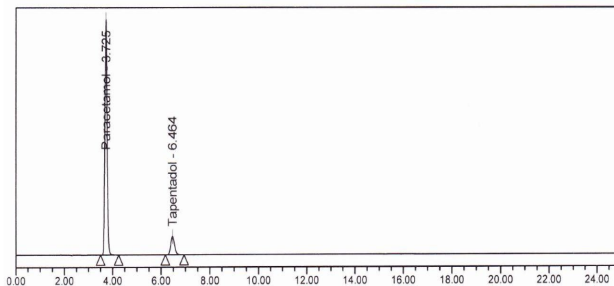
Figure15 : Chromatogram of alkali stressed degradation of drug product
