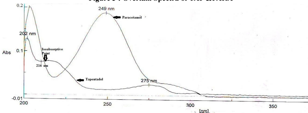
Figure 3 : Overlain Spectra of TAP & PARA
