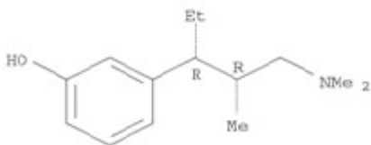
Figure 1 : Structure of Tapentadol
