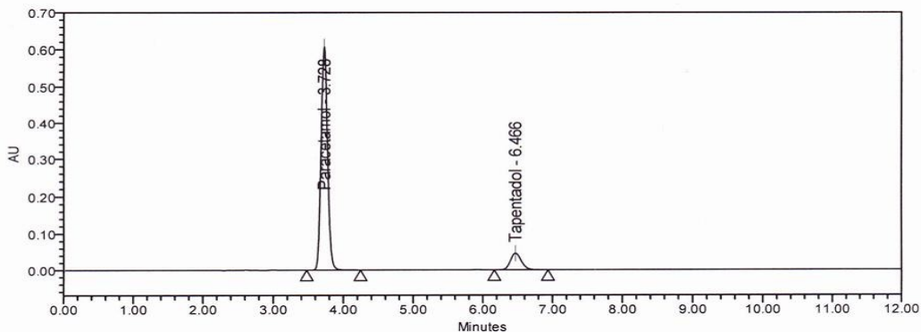
Figure 7: Chromatogram for System Suitability
