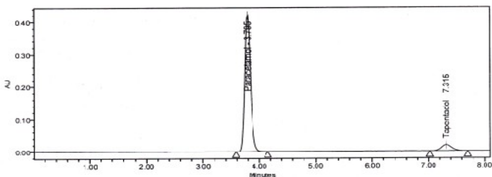
Figure 6: Chromatogram obtained by using Phosphate buffer pH 3.0
