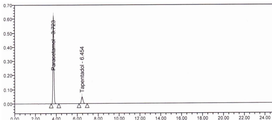
Figure15 : Chromatogram of alkali stressed degradation of drug product
