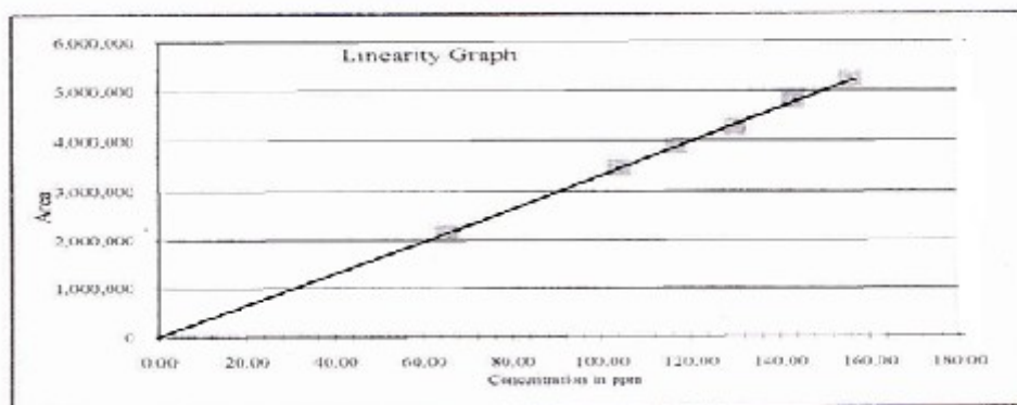
Figure 9: Calibration Curve for PARA
