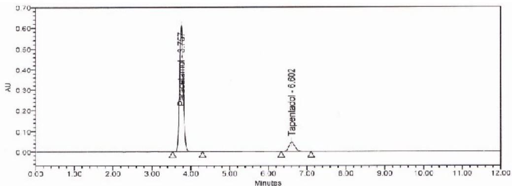
Figure11 :Chromatogram of system precision
