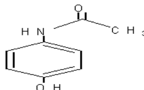
Figure 2 : Structure of Paracetamol
