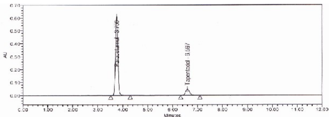
Figure 12 : Chromatogram of Intraday Precision
