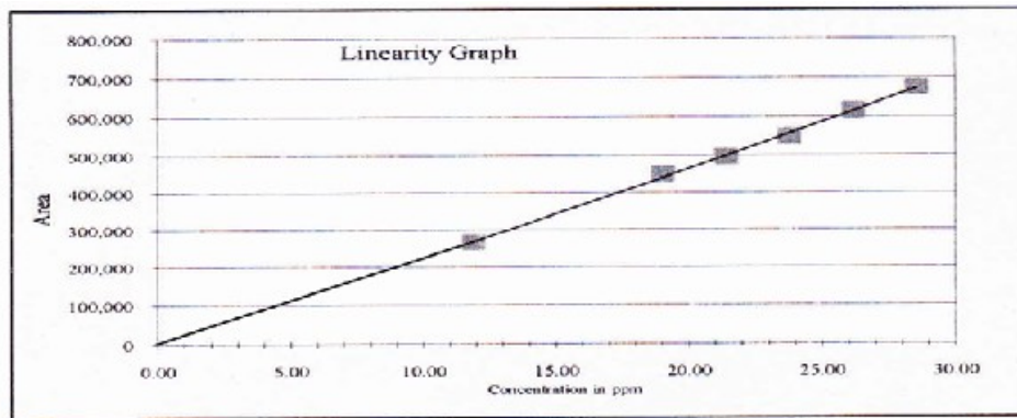
Figure 8 : Calibration Curve for TAP
