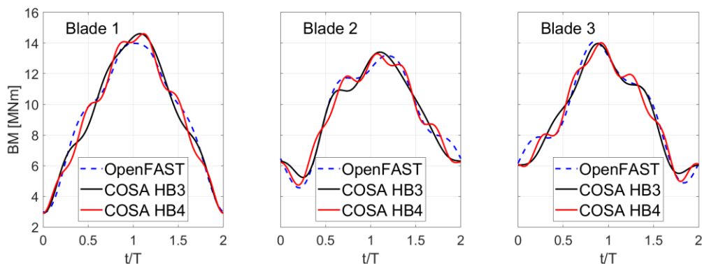
Figure 8. COSA harmonic balance and OpenFAST/AeroDyn predictions of periodic profiles of the out-of-plane bending moment BM on the blades of the pitching NREL 5 MW rotor at \Theta_p=4^\circ .
