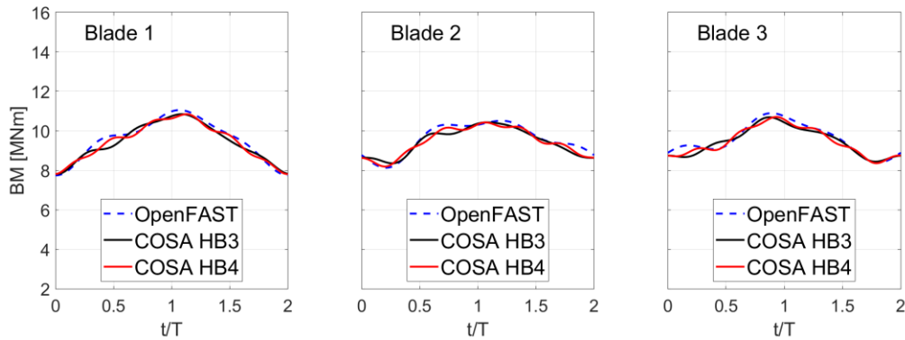
Figure 6. COSA harmonic balance and OpenFAST/AeroDyn predictions of periodic profiles of the out-of-plane bending moment BM on the blades of the pitching NREL 5 MW rotor at \Theta_p=1^\circ .
