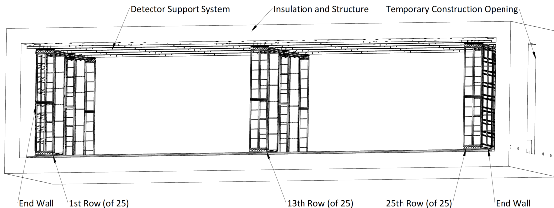
Figure 7.1: Overall model of the SP module showing three of the 25 rows, simplified cryostat, detector support system (DSS) and temporary cryostat opening.
