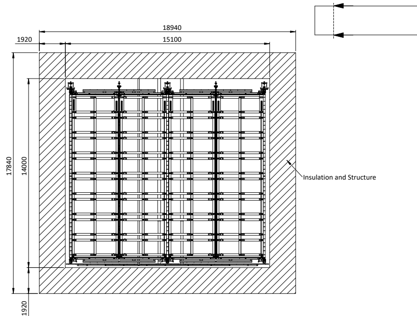
Figure 7.3: Section view of the SP module in the transverse direction.
