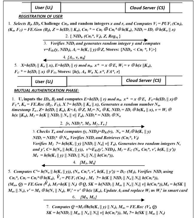
Fig. 2. Proposed Model
