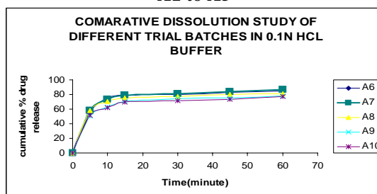
Figure 2 Comparative Dissolution Study of A6 to A10
