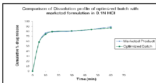
Figure 3 Comparison of dissolution profile of optimized batch with marketed formulation.
