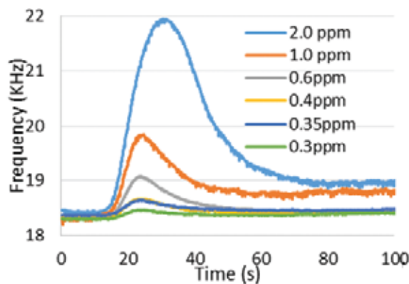
Figure 7. Sensor response at different concentrations of CEES.
