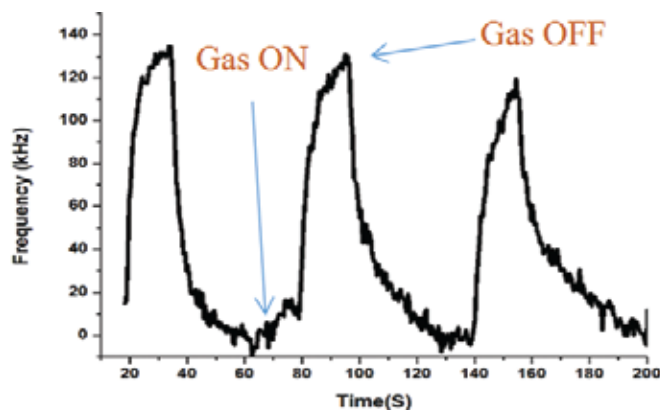
Figure 6. Plot showing frequency versus time for CEES.
