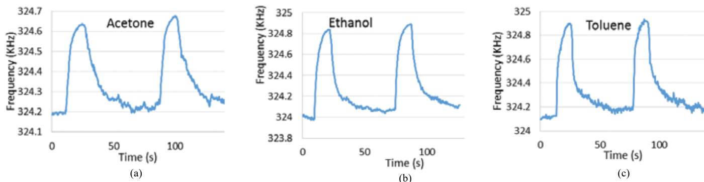
Figure 8. (a) Sensor response for Acetone at 0.5 ppm conc, (b) Sensor response for Ethanol at 0.5 ppm conc, and (c) Sensor response for Toluene at 0.5 ppm conc.
