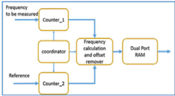
Figure 3. Block diagram of frequency counter.
