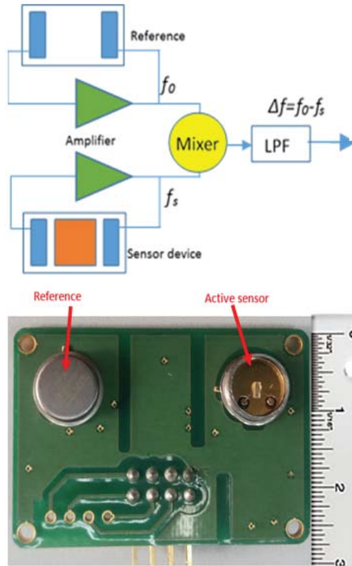
Figure 2. Block diagram and sensor circuit board.
