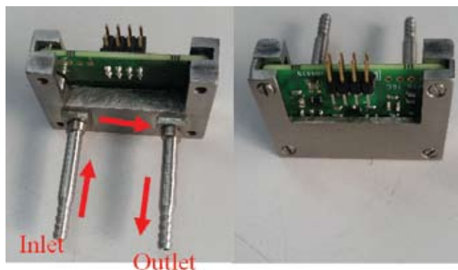
Figure 5. Sensor cell along with circuit board.
