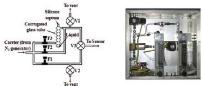
Figure 4. Schematic of vapour generator and vapour generator system.
