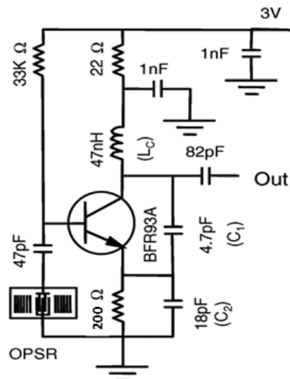
Figure 1. SAW colpitt oscillator circuit.
