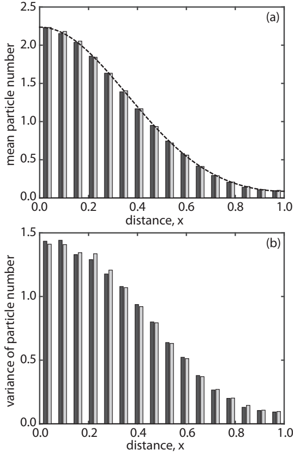
FIG. 3. Comparing the (a) mean and (b) variance of particle numbers for the m = 1 and m = 8 cases at t = 1 , with K = 128/m . Dark gray bars: Results from simulation of the random walk model with m = 1 . Light gray bars: Results from the numerical solution of Eq. (6)/Eq. (7) with m = 8 . Black dashed line in (a): Solution of the limiting diffusion equation.
