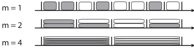
FIG. 1. Representation of particle positions within compartments of different capacity. Shaded cells represent particles, and white cells represent unused capacity. As m increases, the spatial resolution coarsens, and this work reconciles the descriptions at these different scales.
