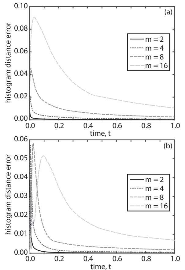
FIG. 4. HDEs for the (a) means and (b) variances in particle numbers as m is varied [22].
