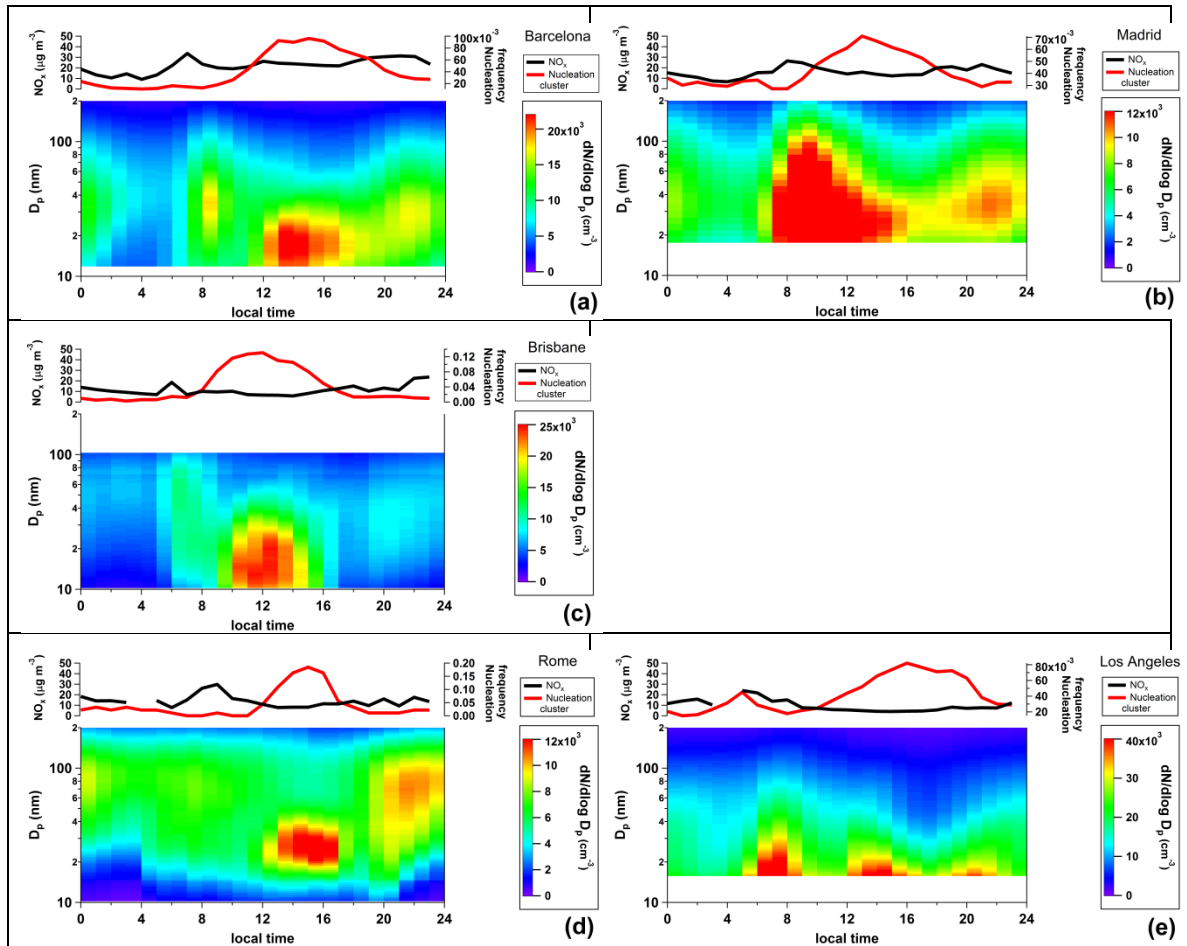
Figure 5: Mean SMPS size distributions on a nucleation day at each selected city, NO x average concentration and the frequency of occurrence of the Nucleation cluster for: a) Barcelona, b) Madrid, c) Brisbane, d) Rome and e) Los Angeles. Please note that NO x concentrations for Madrid represent NO x /2 and for Los Angeles NO x /10. These values are 30-65% lower on nucleation days than the corresponding sampling period average levels.
