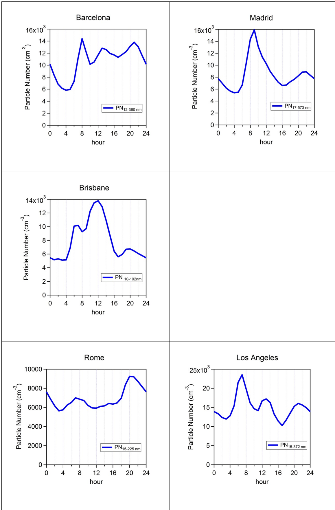
2 Figure S3: Average daily particle number concentration for the study periods at each city.
