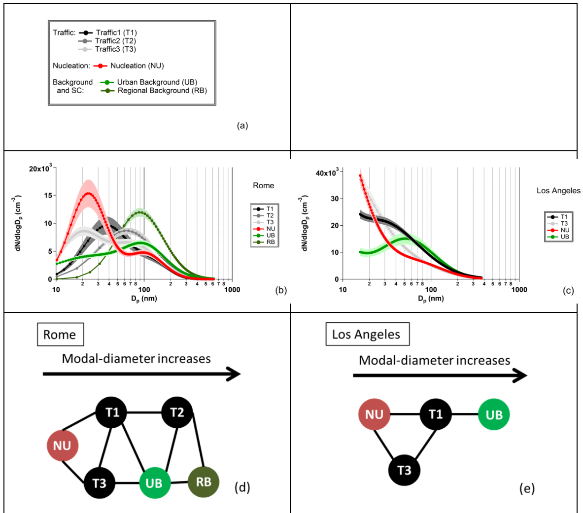
Figure 3: Aerosol size distribution results of the k -Means cluster analysis performed on the SMPS data at the selected complementary cities: a) legend, b) Rome and c) Los Angeles. Shaded areas around the curves represent the confidence limits calculated for 3 sigmas. Please note the different scales for dN/d\log D_p . Cluster proximity diagrams are shown for both cities: d) Rome and e) Los Angeles.
