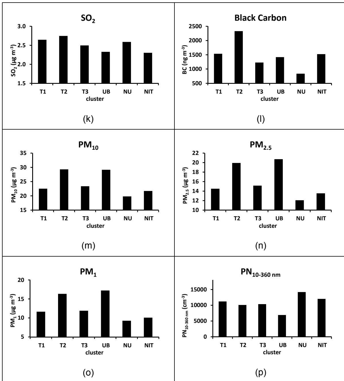
1 Figure S2: Meteorological parameters and gaseous pollutants for the main clusters: a) 2 Temperature, b) Relative Humidity, c) Rain, d) Solar Radiation, e) Wind Speed, f) NO, g) 3 NO 2 , h) NO x , i) O 3 , j) CO, k) SO 2 , l) Black carbon, m) PM 10 , n) PM 2.5 , o) PM 1 , p) PN 10-360 . 4 Although they are extracted from the results for Barcelona, the trend followed by clusters is 5 representative of the rest of the cities.
