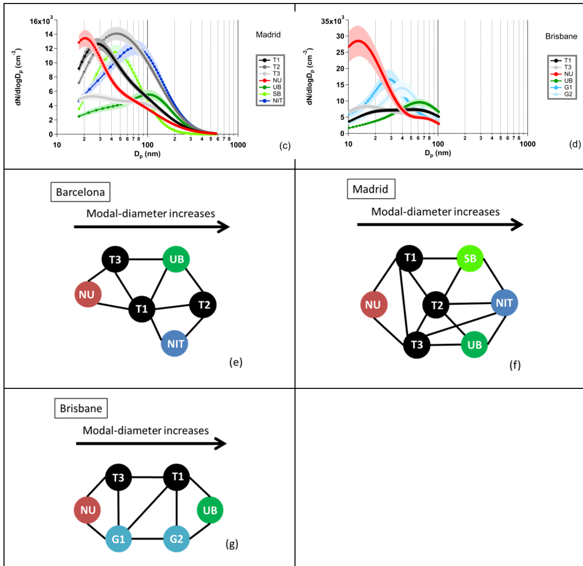
Figure 2: Aerosol size distribution results of the k -Means cluster analysis performed on the SMPS data at each selected city: a) legend, b) Barcelona, c) Madrid, d) Brisbane. Shaded areas around the curves represent the confidence limits \mu calculated for 99.9% confidence level. Please note the different scales for dN/d\log D_p . The corresponding Cluster Proximity Diagram (CPD) is shown for the 3 main selected cities: e) Barcelona, f) Madrid and g) Brisbane.
