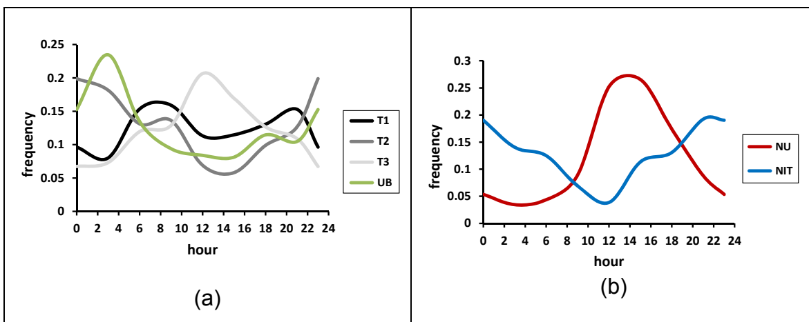
3 Figure S1: Diurnal trends for the main clusters: a) Traffic1 (T1), Traffic2 (T2), Traffic3 (T3) 4 and Urban Background (UB); b) Nucleation (NU) and Nitrate (NIT). Although they are 5 extracted from the results for Barcelona, they are representative of the rest of the cities.
