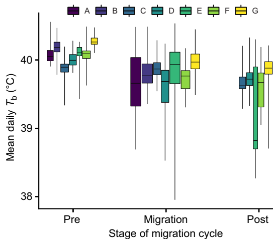
Fig. 3. Bar-headed goose T_b throughout the tracking period. Boxplots showing mean daily T_b at three stages of the tracking period relative to migration ( N = 7 geese pre-migration and during migration, N = 5 post-migration). Boxes show interquartile range, horizontal black line inside the box shows median value, and whiskers show the minimum and maximum T_b per goose. Box width reflects the relative number of days per goose included in each case.
