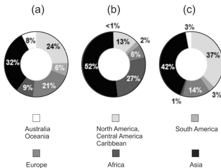
Figure 2. Regional distribution (in per cents) of (a) loss events (total 20,200), (b) fatalities (total 2,275,000), and (c) losses (total USD 3,530 billion in 2011 values) for 1980-2011 (Source: NatCatSERVICE; after Wirtz et al., 2014).
