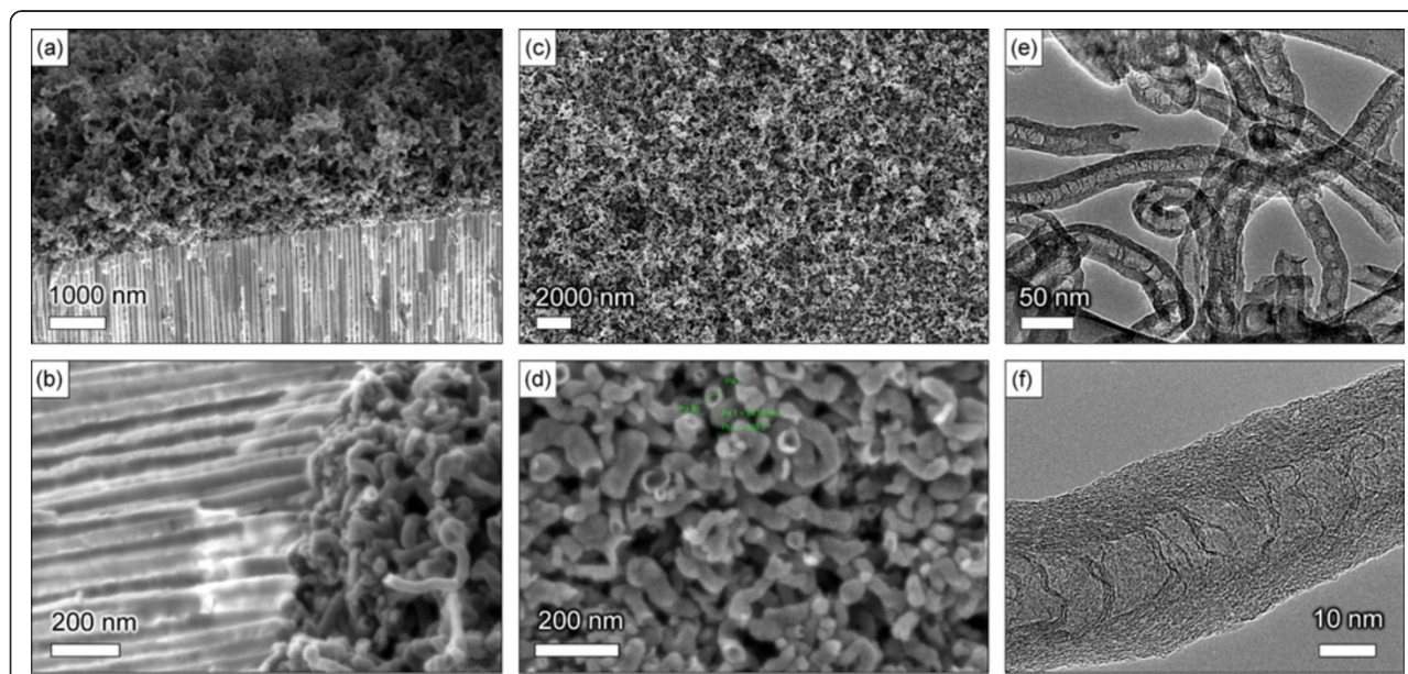
Figure 4 SEM and TEM images of carbon nanotubes grown in 750°C process, Fe only series ( C_2H_4 , no S1813; Table 1). (a, b) Side view, nanotubes are present on the membrane top only, the channels are empty; (c, d) top view; and (e, f) the multi-walled nanotubes contain approximately 25 to 30 walls.
