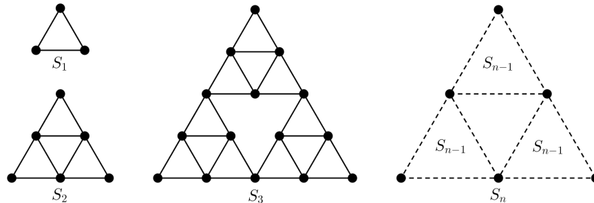
Figure 1. Sierpiński gasket graphs.
