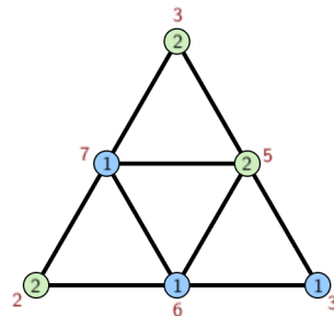
Figure 2. A sigma coloring of S_2 .
