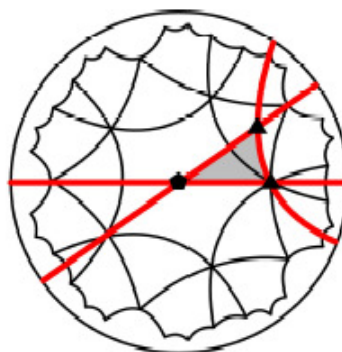
Figure 7: Finding symmetries of the 5 \cdot 3 \cdot 5 \cdot 3 \cdot 5 \cdot 3 tiling on a fundamental triangle [7]
