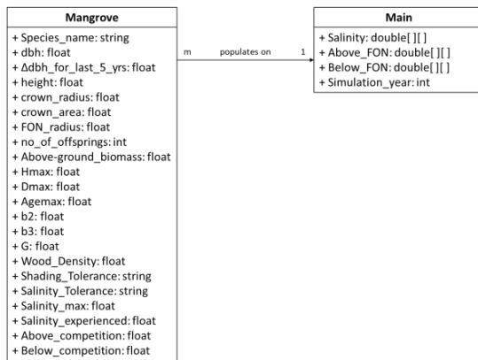
Figure 2: Class diagram of the mangrove forest stand model.
