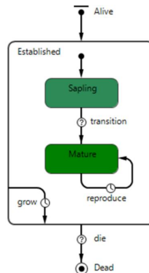
Figure 3: The statechart of the mangrove agent. Processes represented by a clock icon are executed every time step while processes represented by a question mark icon are executed only when specific conditions become true.
