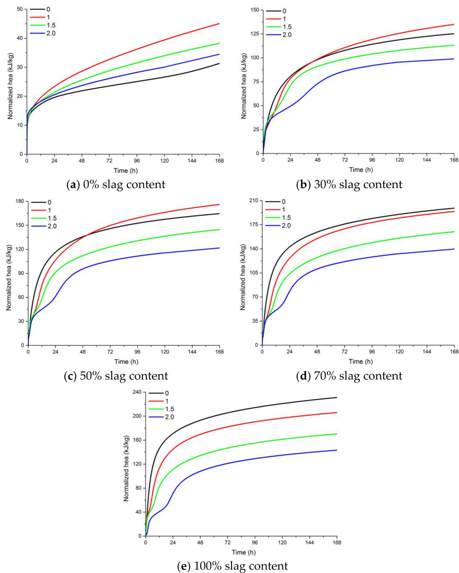
Figure 7. The effect of the activator modulus and slag content on the cumulative heat release of AAFS. (a) 0% slag content; (b) 30% slag content; (c) 50% slag content; (d) 70% slag content; (e) 100% slag content.
