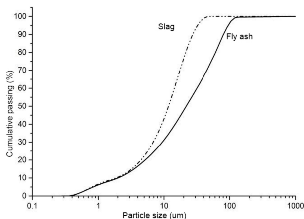
Figure 1. Particle size distribution of fly ash and slag.
