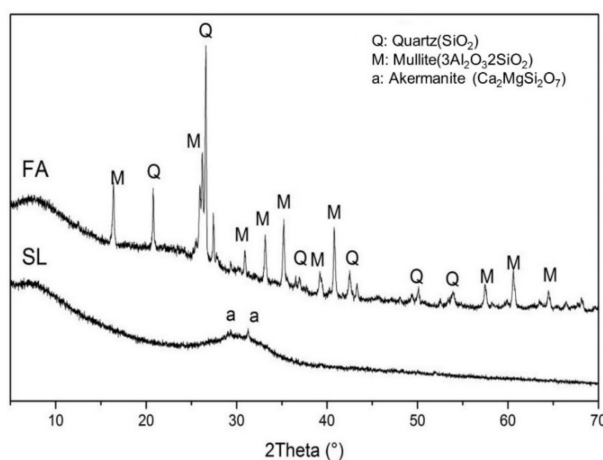
Figure 2. X-ray diffraction analysis of the fly ash and the slag.
