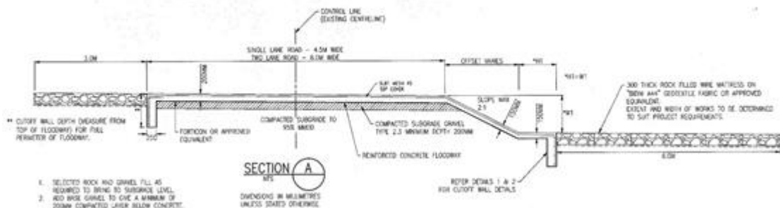
Figure 1 Cross section of floodway Type 2
