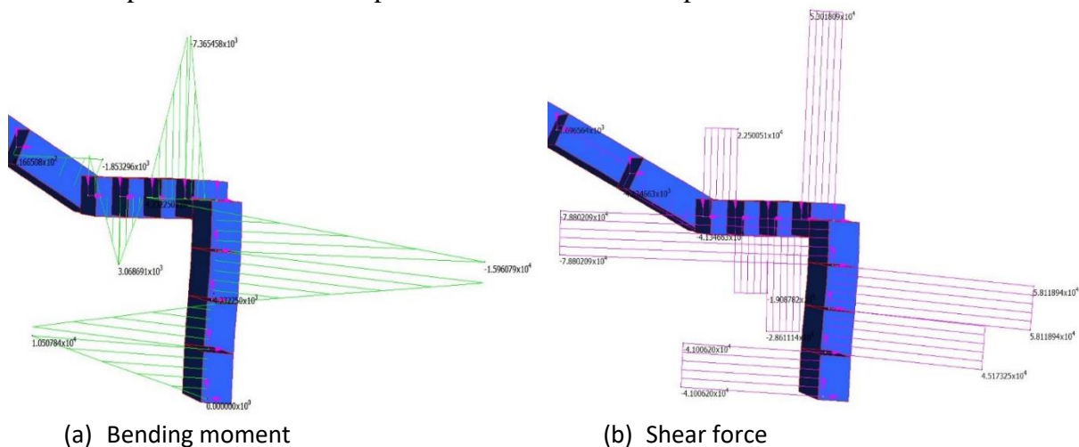
Figure 7 Sample of 2D frame model for M^* and V^* distribution
