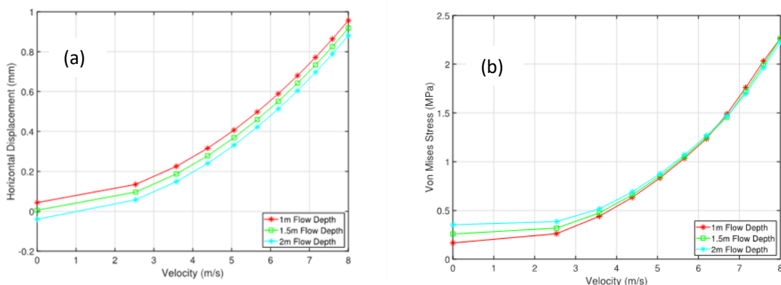
Figure 4 Horizontal displacement and Von Mises stress with increasing flow depth and velocity
