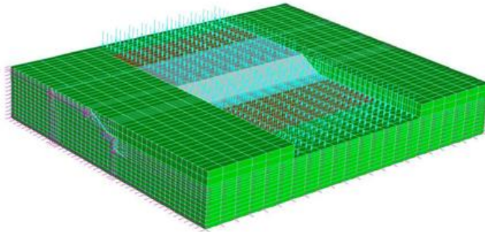
Figure 3 Floodway model with medium mesh size
