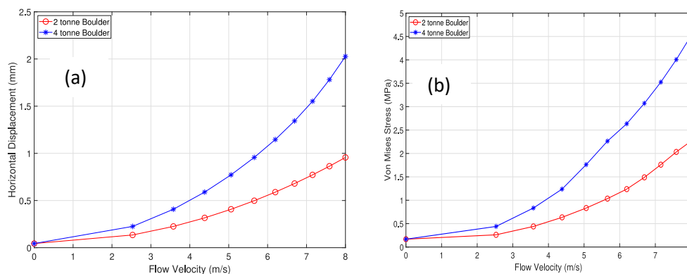
Figure 5 Effect of 2 and 4 tonne boulder impact
