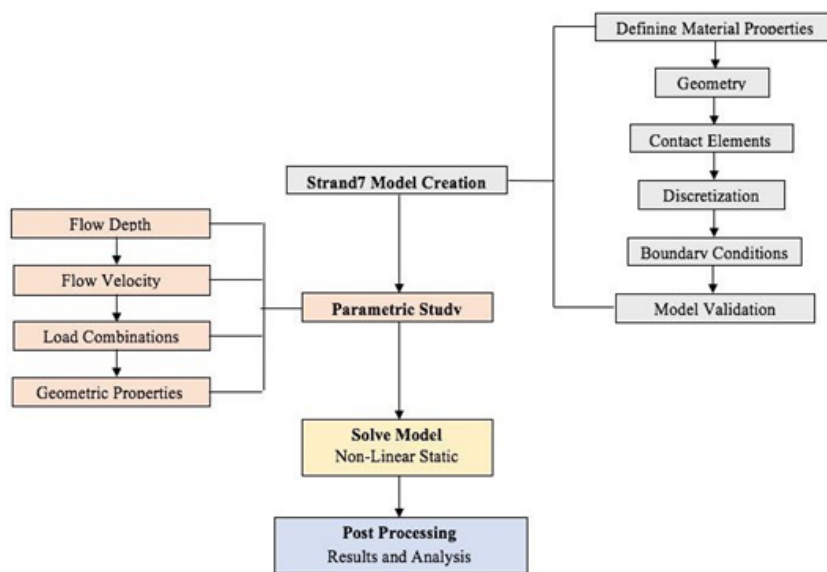
Figure 2 Modelling process
