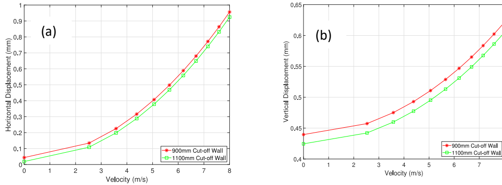
Figure 6 Effect of 2 cut off wall configurations
