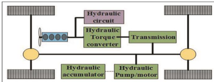
Figure 4. Series-Parallel Powertrain Configuration (Wang et al., 2016, p.3)
