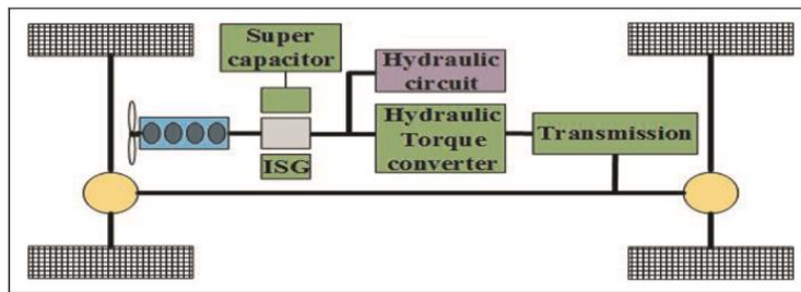
Figure 3. Parallel Powertrain Configuration (Wang et al., 2016, p.3)
