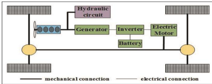
Figure 2. Series Powertrain Configuration (Wang et al., 2016, p.3)
