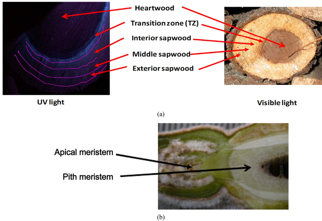
Figure 1. (a) Cross-section of a black walnut stem under white light. The transition zone fluoresces blue under UV light; (b) The location of the pith meristem region in a branch of black walnut.
