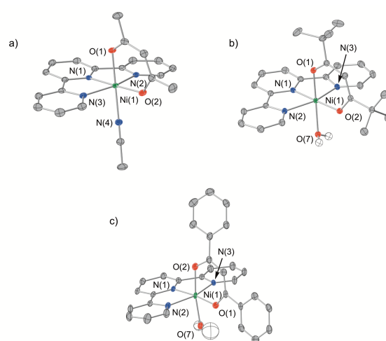
Figure 1 Cationic portions of a) 1 , b) 2 and c) 3 . Hydrogen atoms except for those of coordinated water molecules have been omitted for clarity. Ellipsoids are plotted at the 50% probability level.
