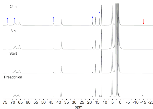
Figure 5 ^1\text{H} -NMR spectra of 1 in dry \text{CD}_3\text{CN} with 10% \text{D}_2\text{O} (v:v) and excess \text{NEt}_3 (5 eq) over time, starting with a preaddition spectrum ( \text{NEt}_3 and \text{D}_2\text{O} not added) (a), a spectrum after addition of all reagents (b), 3 hours later (c) and 24 hours later (d). The blue arrow highlights the growth of 4 , and the red arrow represents the disappearance of the diketonate C-H proton.
