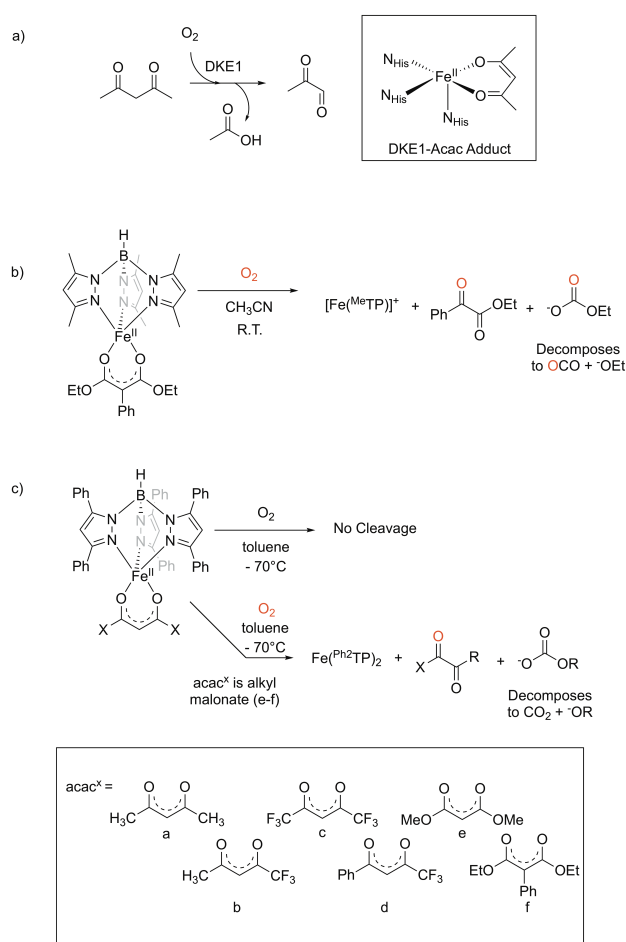
Scheme 1 a) Reaction catalyzed and active site iron center of DKE1. b) Diethylphenylmalonate-containing model complex for the active site of DKE1. c) Complexes with diketonates e-f undergo oxidative C-C bond cleavage whereas those with diketonates a-d do not exhibit this reactivity.
