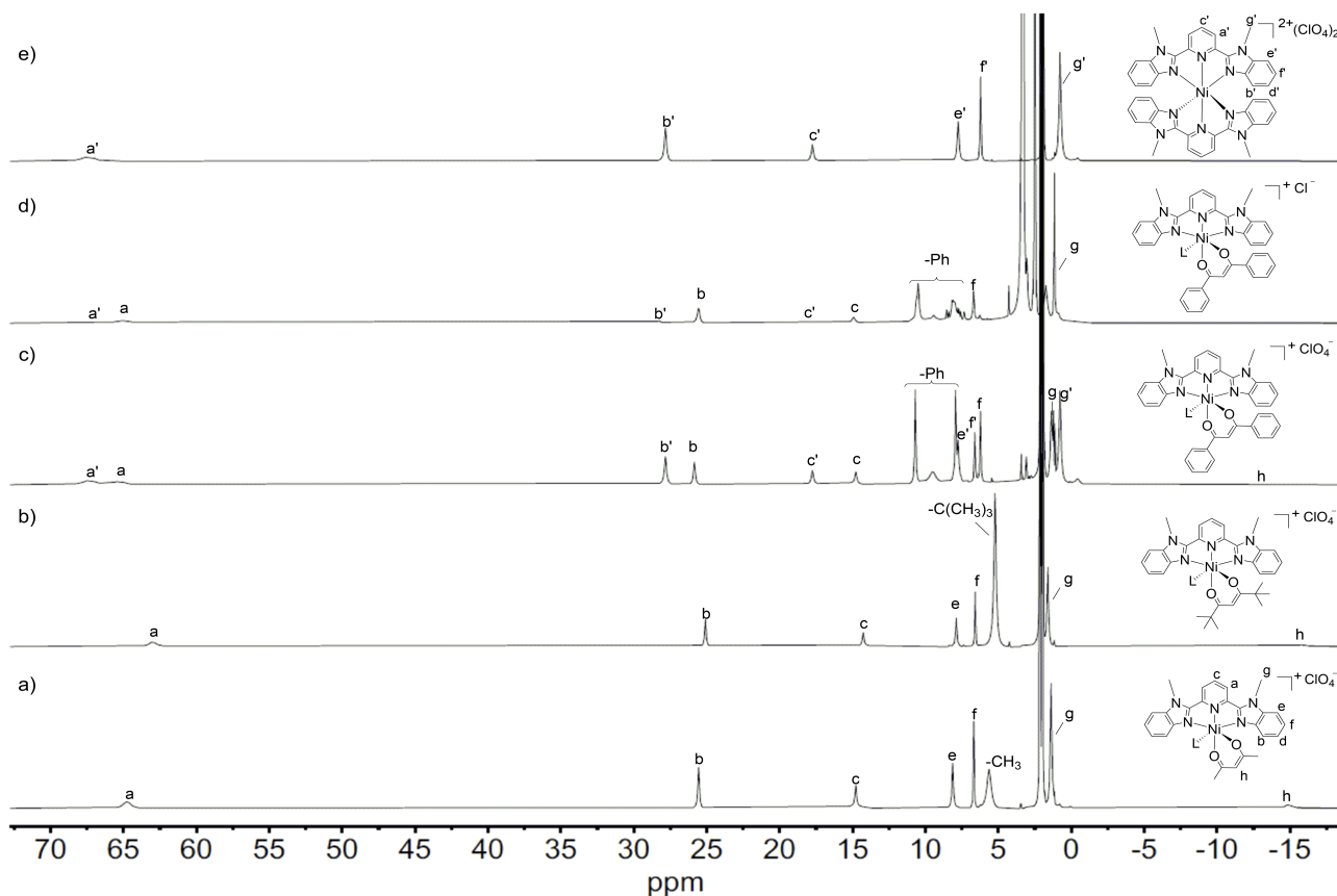
Figure 3 ^1\text{H} NMR spectra of MBBP-ligated a) 5 , b) 6 c) 7-ClO 4 , d) 7-Cl and e) 8 in \text{CD}_3\text{CN} .
