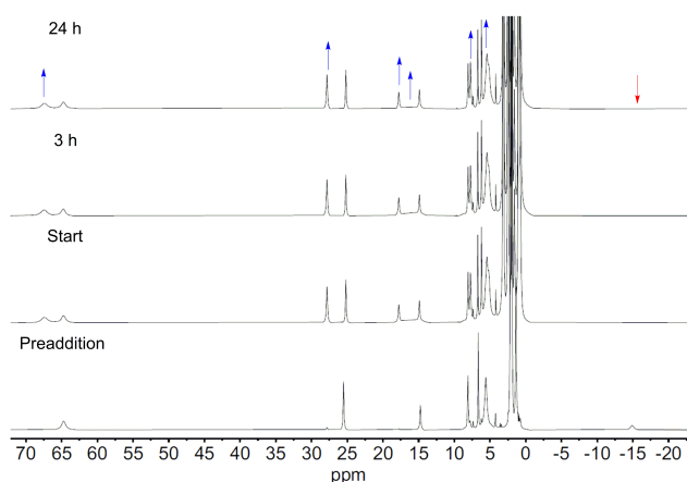
Figure 6 1 H-NMR stacked spectra of 5 in CD 3 CN with 10% D 2 O and excess NEt 3 over time, starting with a pre-addition spectrum (NEt 3 and D 2 O not added) (a), a spectrum after addition of all reagents (b), 3 hours later (c) and 24 hours later (d). The blue arrow highlights the growth of 8 , and the red arrow represents the disappearance of the α proton.
