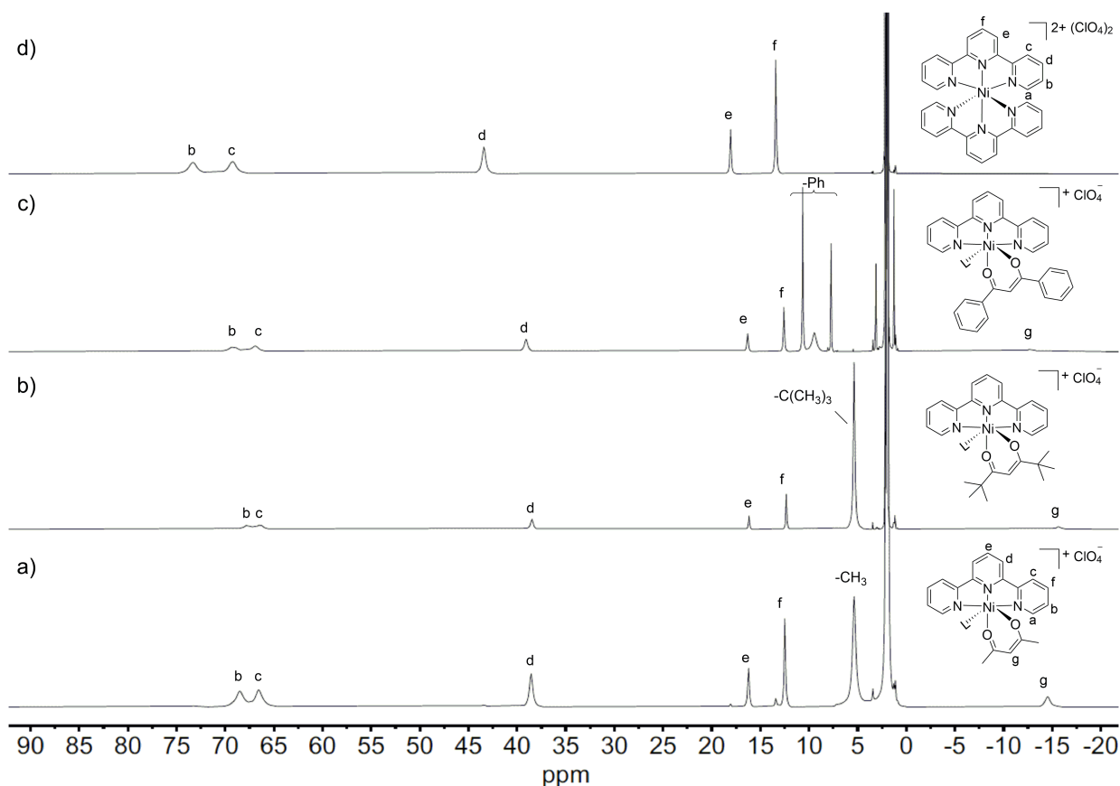
Figure 2 ^1\text{H-NMR} spectra of TERPY-ligated a) 1 , b) 2 , c) 3 and d) 4 in \text{CD}_3\text{CN} .
