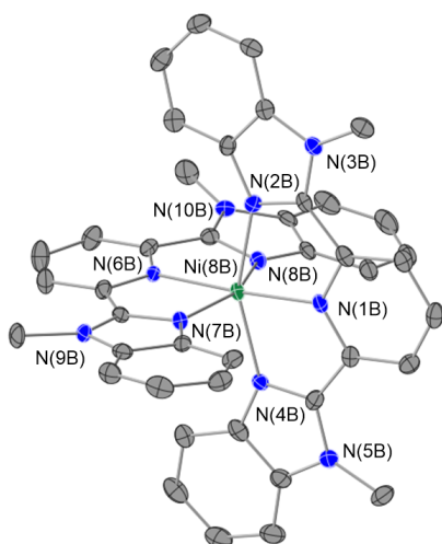
Figure 4 Thermal ellipsoid representation of a cationic portion of the X-ray structure of 8 . The complex crystallizes with two cations per asymmetric unit. Hydrogen atoms have been omitted for clarity. Ellipsoids are plotted at the 50% probability level.
