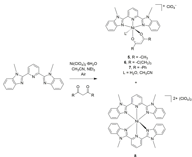
Scheme 5. Products identified in the syntheses of 5-7 . Complex 8 was identified in each reaction mixture using ^1\text{H} NMR based on an independently generated sample.
