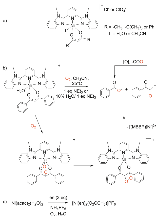
Scheme 3 a) MBBP-ligated Ni(II) diketonate complexes reported by Ramasubramanian, et al. 24 b) Proposed pathway of \text{O}_2 reaction of MBBP-ligated Ni(II) phenyl diketonate complex. c) Oxidative cleavage of an acetylacetonate ligand. 25
