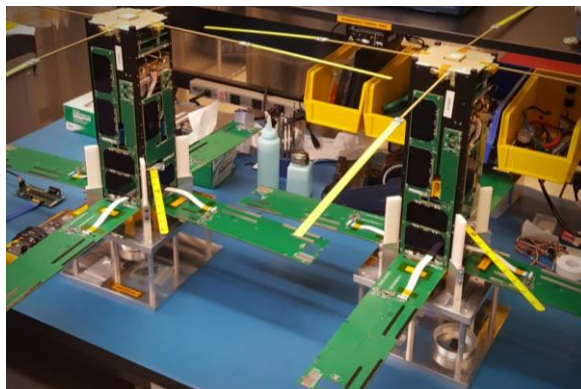
Figure 2: Both TBEx satellites at the University of Michigan prior to launch vehicle integration
