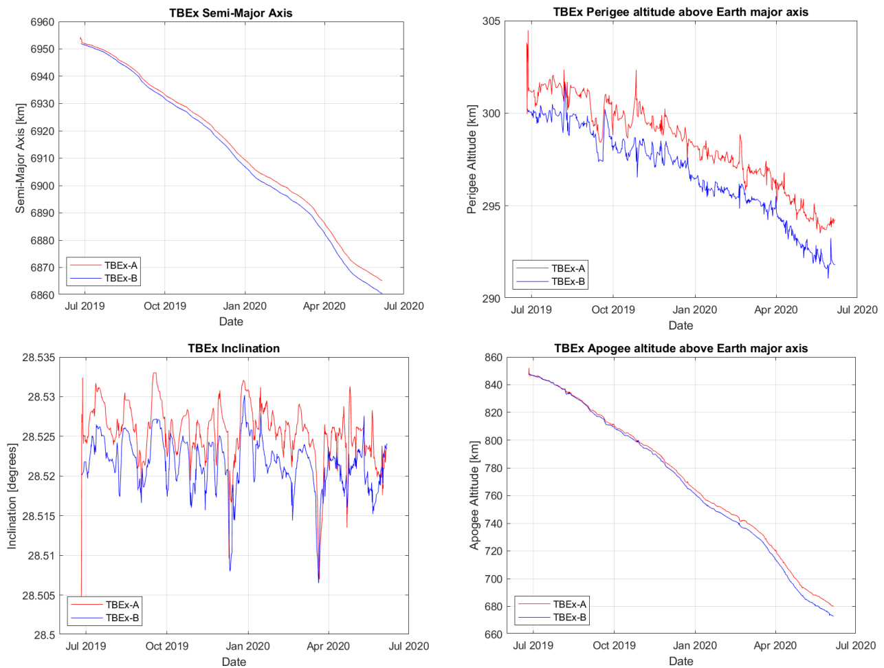
Figure 3: Several orbital parameters of the TBEx satellites over time. Note the similarity between the orbits of the two spacecraft
