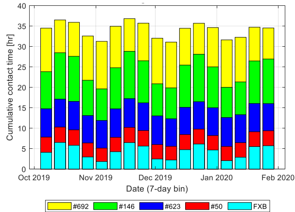
Figure 5: Weekly total contact time between TBEx-B and the augmented network. Colored bars indicate the amount of contact time gained per week by the addition of that station into the network. Stations #2 and #853 do not appear because they are temporally eclipsed by the others. Stations were added in order of increasing geographical distance from the FXB
