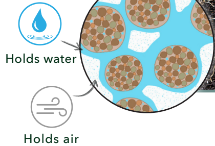
Soil Particles
