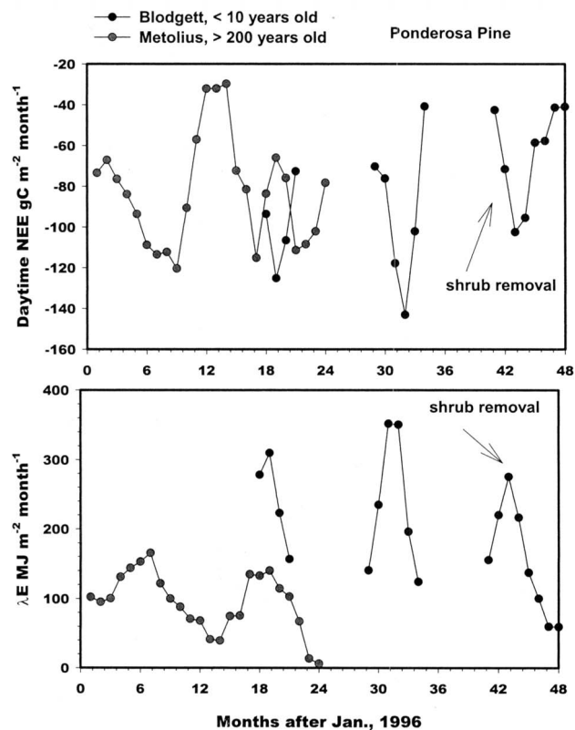
FIG. 13. The impact of stand age on daytime CO_2 exchange (NEE) and latent heat exchange (LE). The data are from a young (< 10 yr; black circles) and an old (> 200 yr; gray circles) ponderosa pine forest (see Law et al. 2001, manuscript submitted to Global Change Biol. ; Goldstein et al. 2000).
