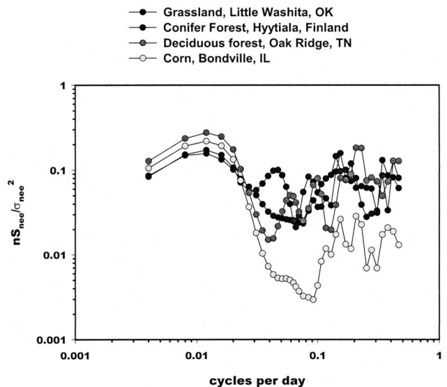
FIG. 7. Power spectrum of \text{CO}_2 flux over the course of a year at sites of contrasting climate, functionality, and structure. Power spectra for the other sites were derived from time series of 1 yr in duration. The power spectra on the y axis are multiplied by natural frequency ( n ) and are normalized by variance.
