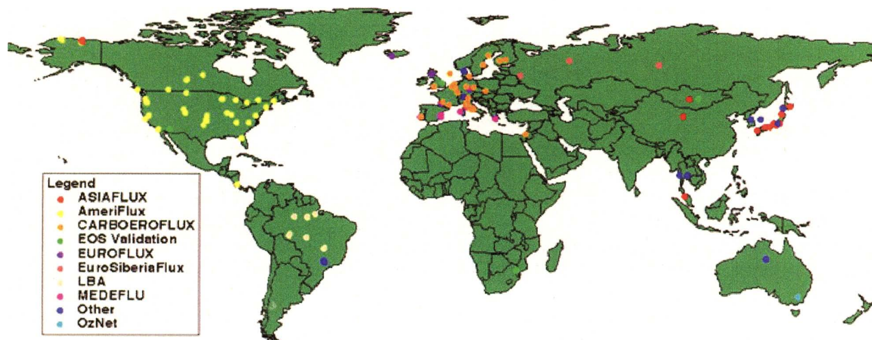
FIG. 1. Global map of FLUXNET field sites.
