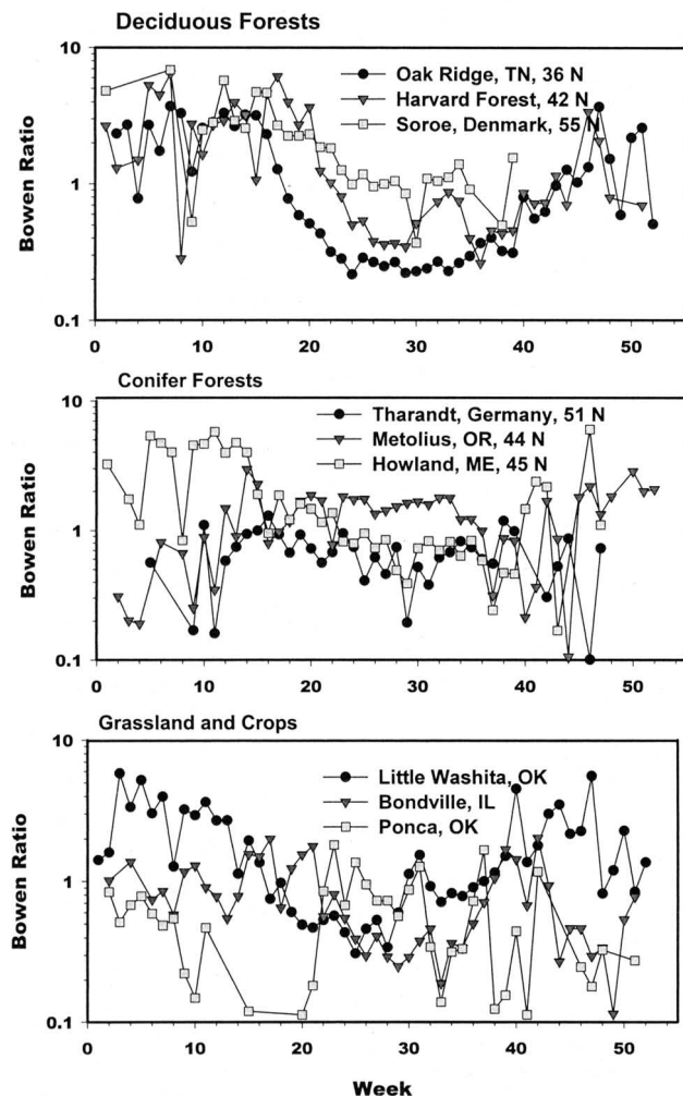
FIG. 10. Seasonality of Bowen ratio, the ratio between sensible and latent heat flux densities, at representative deciduous forests, conifer forests, and grassland and crop sites.
