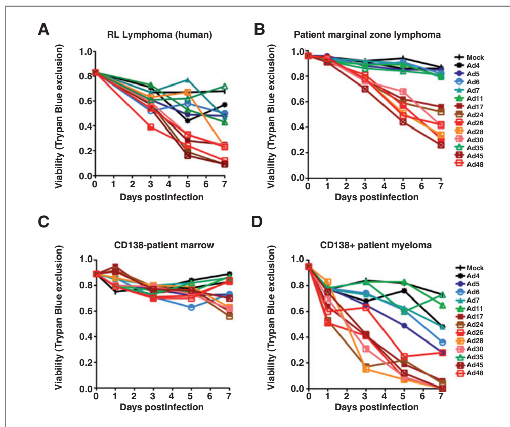
Figure 4. Expanded comparison of adenoviral serotypes for infection and replication in B-cell cancer cells. A 13-member panel of adenoviral serotypes are tested against 2 B-cell cancers. Lymphoma: A, RL human lymphoma; B, patient marginal zone lymphoma. Myeloma: C, nonmalignant CD138– patient bone marrow cells; D, malignant CD138+ patient bone marrow cells. Viability was assessed by Trypan Blue uptake following infection at an MOI of 10,000 viral particles/cell. Green, species B; blue, species C; yellow, orange, red, species D; and brown, species E.
