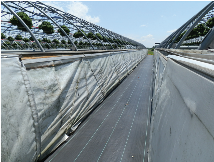
Figure 7. Drop down sidewalls ( above and adjacent ) are preferred since ventilation occurs above the plants rather than near the ground, which can slow plant growth and increase the potential for cold injury.
