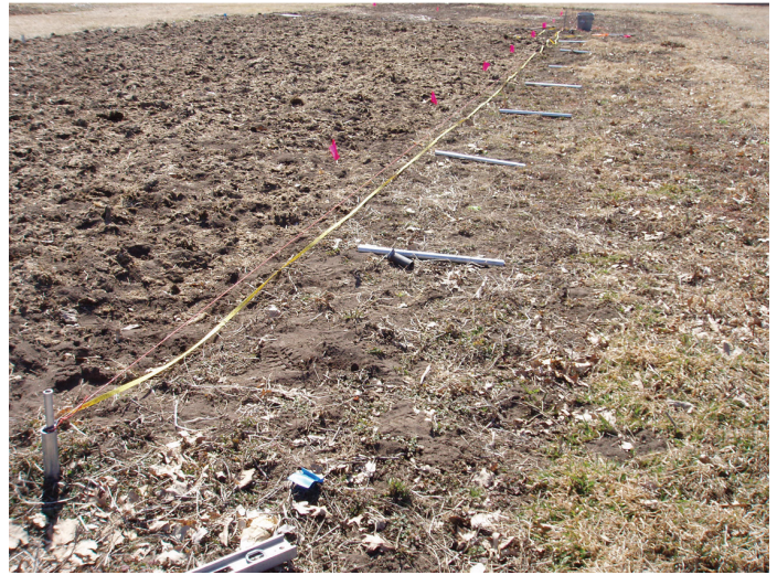
Figure 13. Use of a string line and marking flags to identify ground post locations.
