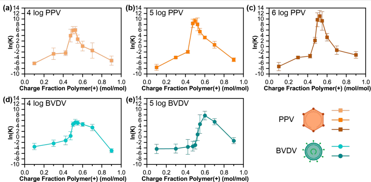
Figure 5. Partition coefficient as a function of the polymer charge fraction associated with cationic K_{400} for coacervates prepared with different concentrations of (a-c) PPV and (d,e) BVDV. All data points are the average of three separate tests, and error bars represent the standard deviation.
