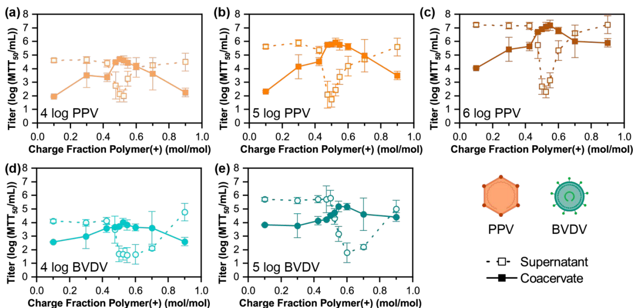
Figure 4. Live virus titration as a function of the polymer charge fraction associated with cationic K_{400} for both the supernatant (open symbols) and coacervate (closed symbols) phases for samples prepared with different total starting concentrations of (a-c) PPV and (d-e) BVDV. All data points are the average of three separate tests, and error bars represent the standard deviation.
