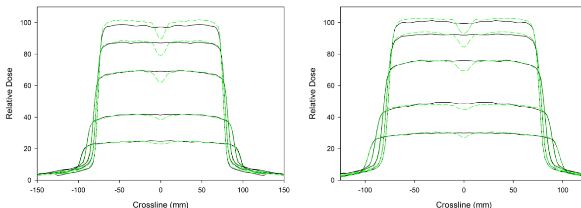
Figure 2. Cross profiles with (green) and without (black) the IMP at depths of 2, 5, 10, 20 and 30 cm for (a) 6MV and (b) 10MV photons.
