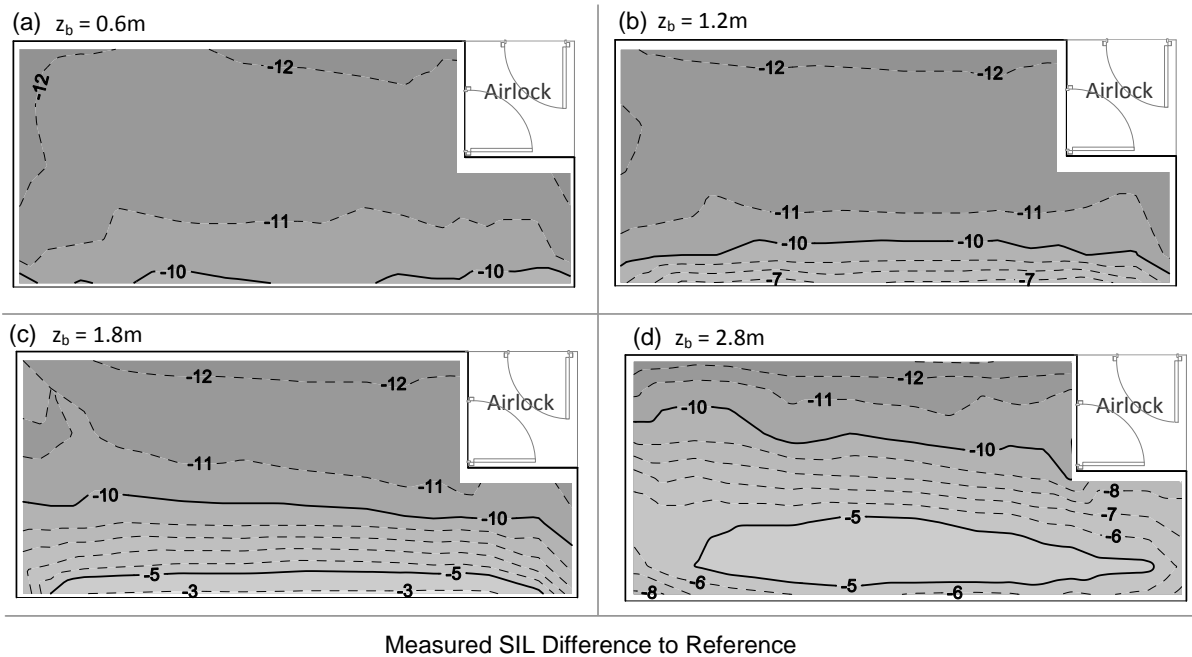
Figure 6: \Delta SIL_{meas} contours over horizontal planes (a) z_b=0.6m , (b) z_b=1.2m , (c) z_b=1.8m , and (d) z_b=2.8m .
