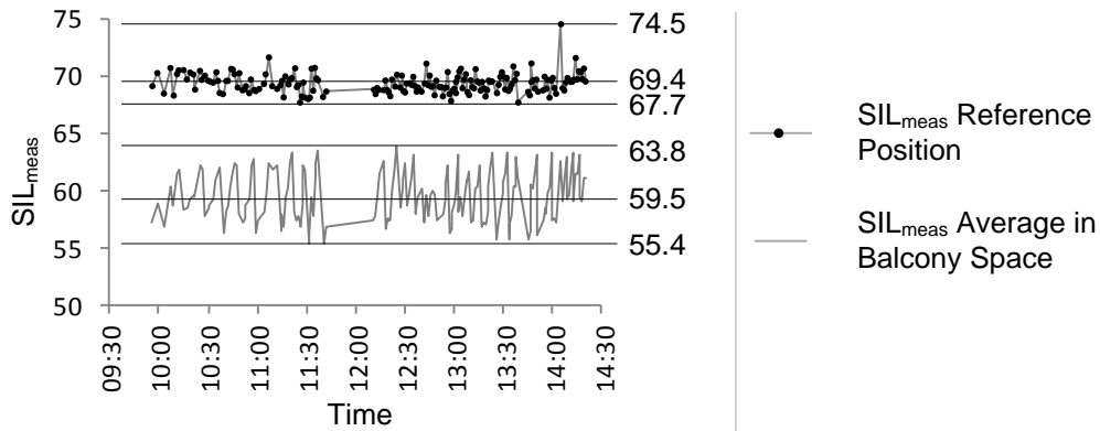
Figure 5: SIL_{meas} at the reference position and the average SIL_{meas} across all receivers within the balcony space.
