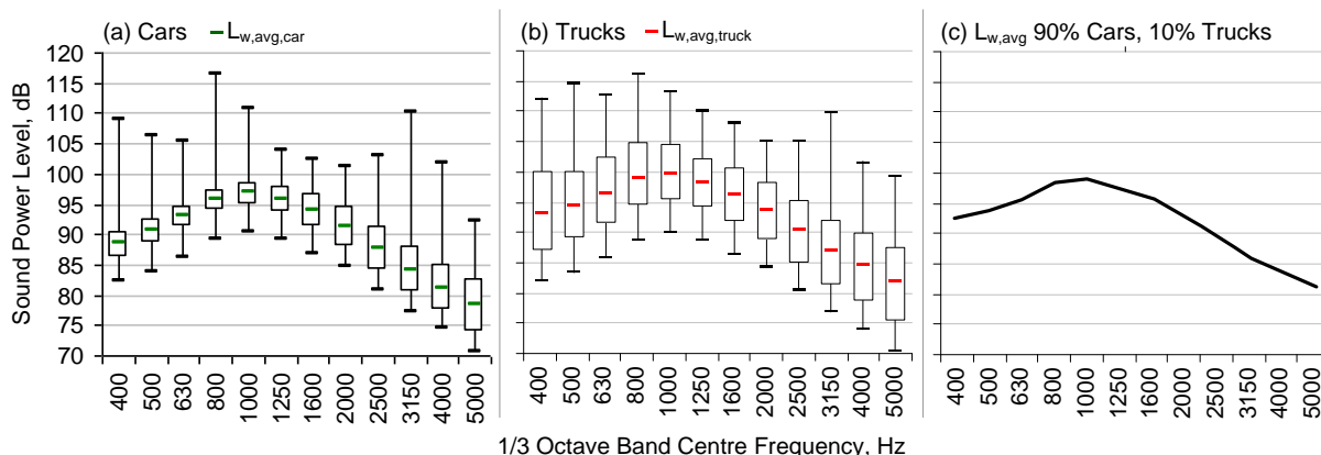
Figure 4: Spread of measured sound power levels using quartile plots and arithmetic average per vehicle classification (a) cars, (b) trucks and (c) L_{w,avg} 90% cars, 10% trucks (color online).
