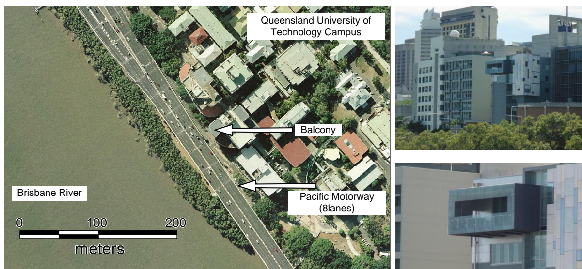
Figure 1: Measurement site location and environment and theoretical model extents. Balcony located at coordinates 27°28'40.75"S, 153°01'38"E.
