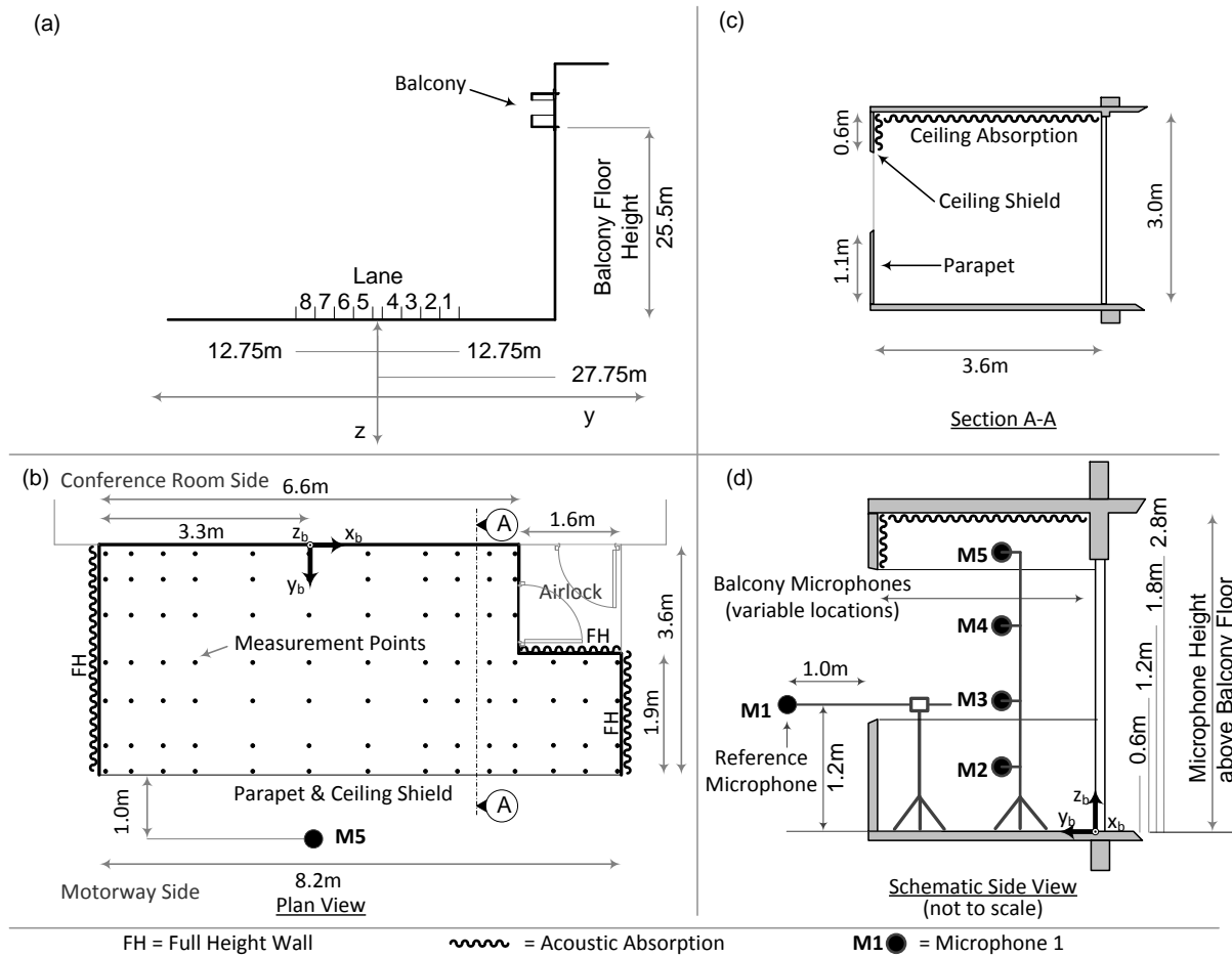
Figure 2: Site and model geometry, (a) dimensions of the street and balcony location, (b) plan view of balcony with relevant dimensions and showing microphone locations in horizontal plane, (c) section view of balcony with relevant dimensions, and (d) section view showing microphone locations designations and vertical locations.
