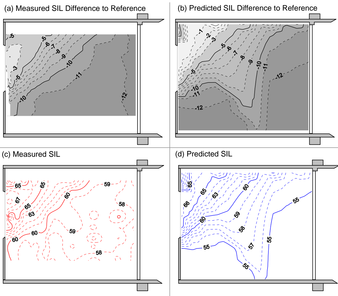
Figure 7: Measured and calculated SIL contours in central vertical plane (a) \Delta SIL_{meas} , (b) \Delta SIL_{pred} , (c) SIL_{meas} , and (d) SIL_{pred} (color online).
