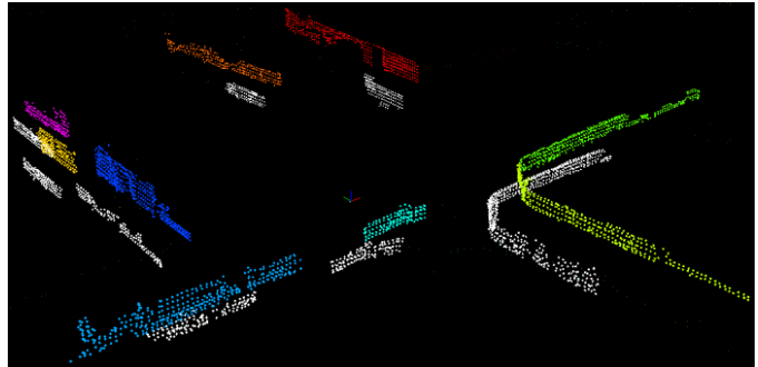
Fig. 1: An illustration of the presented loop-closure detection framework. The planes of the current keyframe are shown below (in white), and the corresponding planes of the keyframe in the map are shown above. Colors are used to indicate the point cloud plane segmentation.
