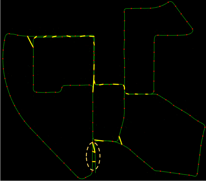
Fig. 7: Illustration of loop-closure detection with LiPMATCH: the figures show loop-closures detected in real time during sequence 00 of the KITTI dataset. The trajectory is before pose graph optimization. The red dots represent locations where plane extraction and loop-closure detection were performed and the yellow lines indicate the detected loops.
